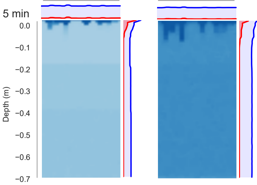
(a) Simulation of 40 mm irrigation in 0.5 h 15 vol.% 31 vol.%
