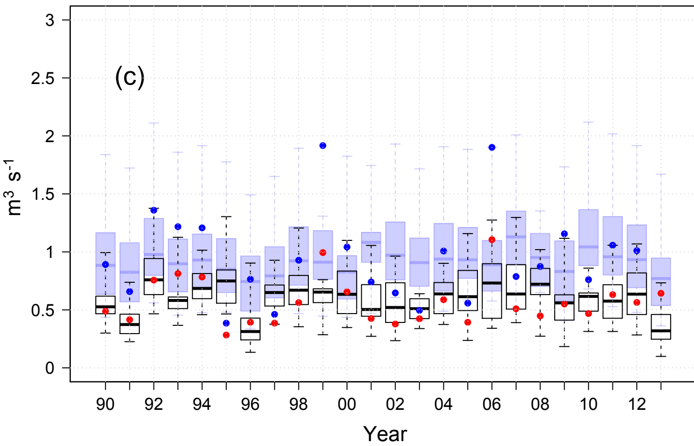
Station 21 RAW CRPSS = 0.54 CRPSS.s = -0.41
