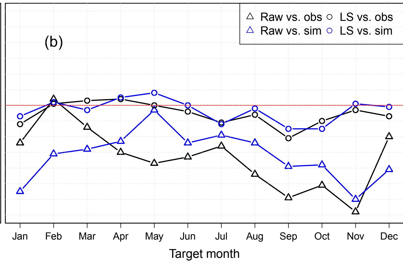
Station 21 LS CRPSS = -0.04 CRPSS.s = -0.05
