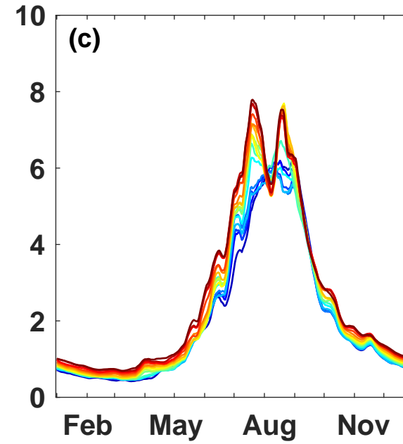
TVP - HBV
