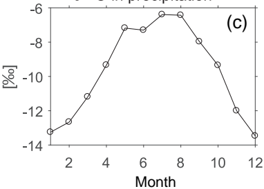
\delta^{18}\text{O} in precipitation
