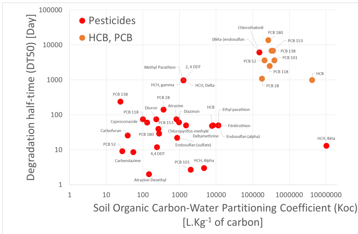
Figure S1: Half-life time (DT50) of 38 legacy and modern organic chemical pollutants (including 30 pesticides, the hexachlorobenzene and 7 polychlorinated biphenyls) as a function of soil organic carbon-water partitioning coefficient (Koc)
