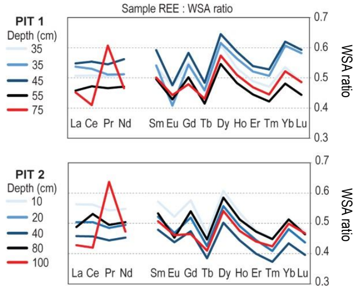
Figure S3: Change of rare-earth elemental composition with depth (based on the World Shale Average (WSA) standard) for pit 1 and pit 2.
