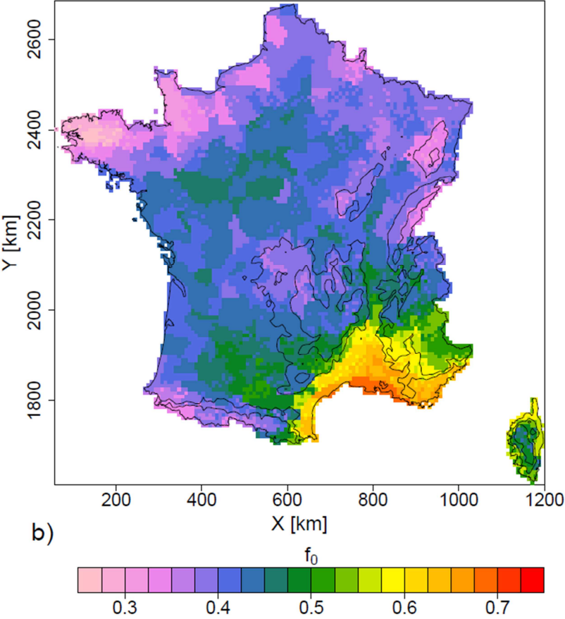
Figure S1: Probability of dry days (1982-2001). A day is considered to be dry if the precipitation amount for this day is smaller than 0.1mm.
