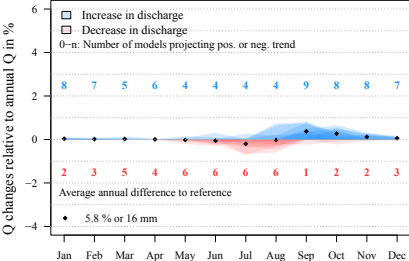
(a) RCP 4.5 (2030–2059)
