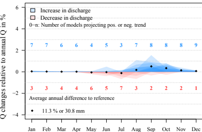
(c) RCP 8.5 (2030–2059)
