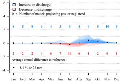
(b) RCP 4.5 (2070–2099)
