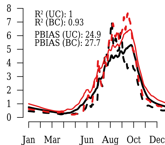
EC-EARTH-RACMO
