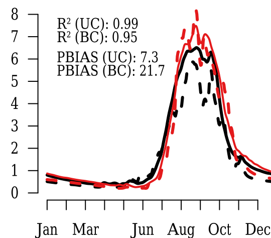
MPI-M-ESM-LR-RCA4
