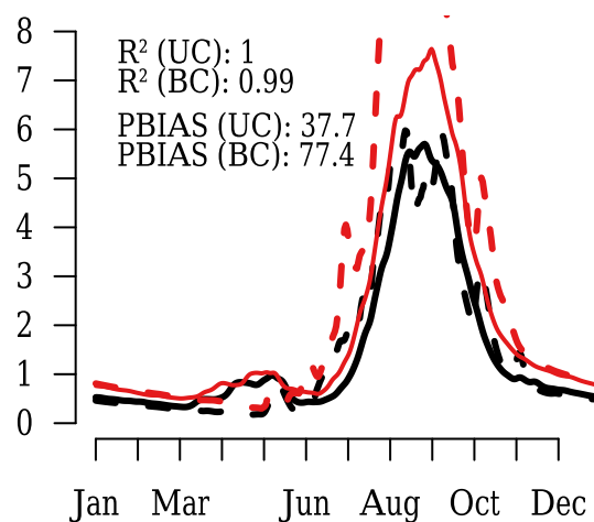
MIROC-RCA4
