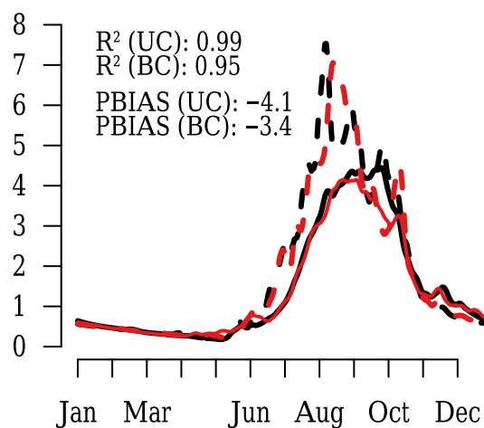
GFDL-RCA4
