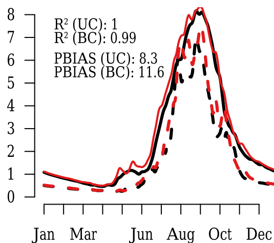
EC-EARTH-RCA4
