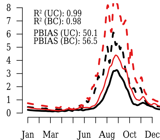
CNRM-CM5-RCA4
