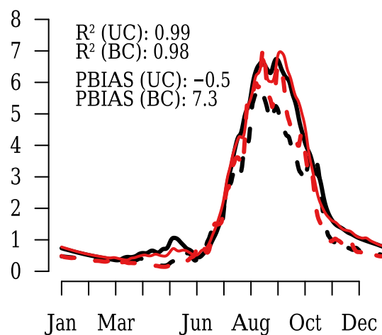
EC-EARTH-Hirham5
