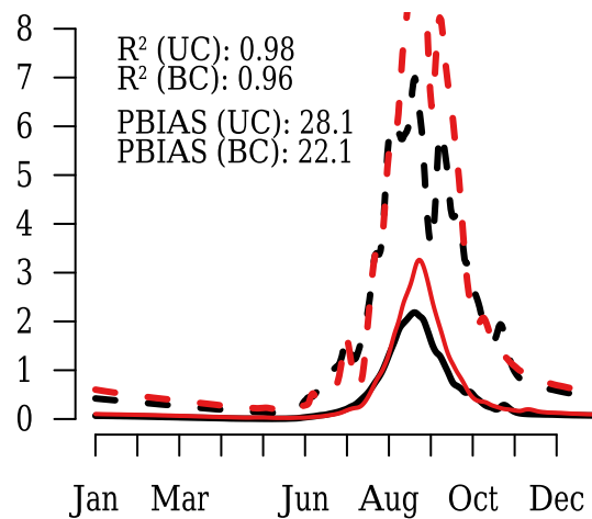
CanESM2-RCA4
