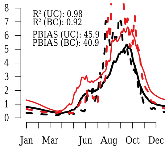
CanESM2-RCM4
