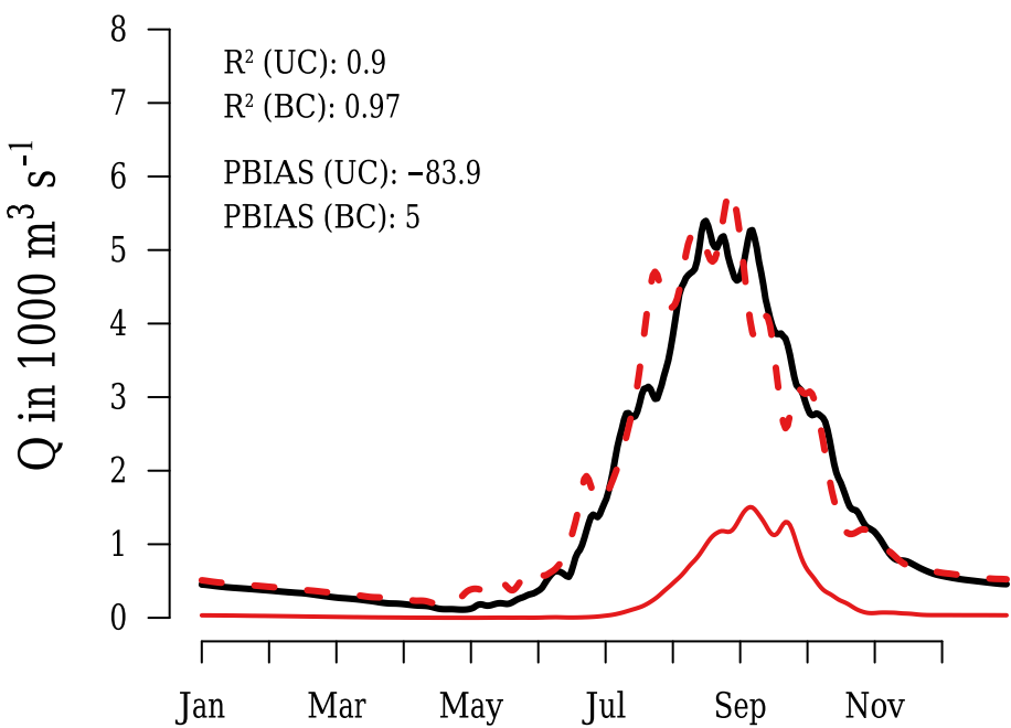
IPSL
