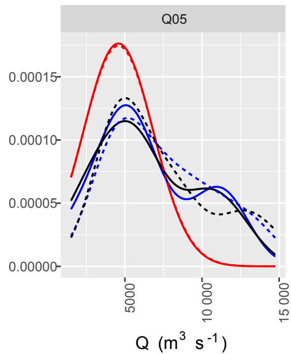
Flows exceeded 5 % of time
