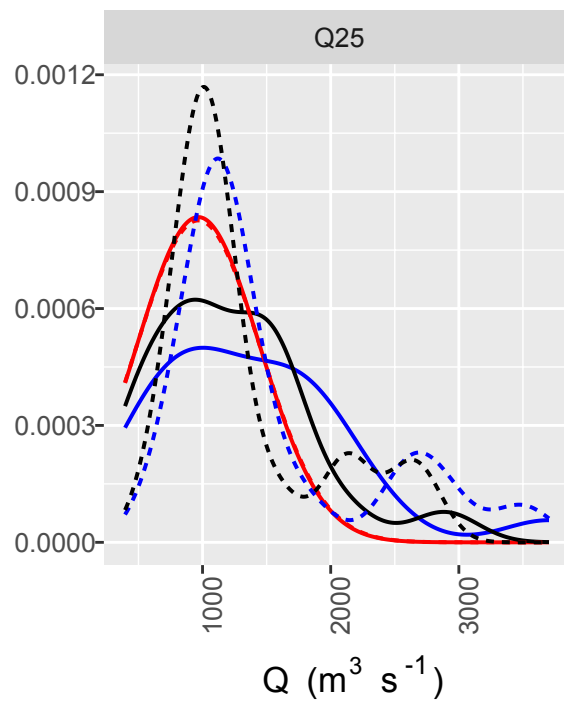
Flows exceeded 25 % of time
