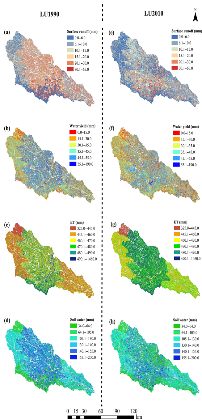
Figure 7. Simulated spatial distribution of surface runoff, water yield, ET, and soil water under land use change between 1990 (a–d) and 2010 (e–h).
