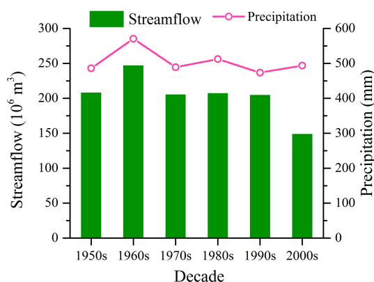
Figure 2. Precipitation and streamflow changes in different decades in the Yanhe Basin.
