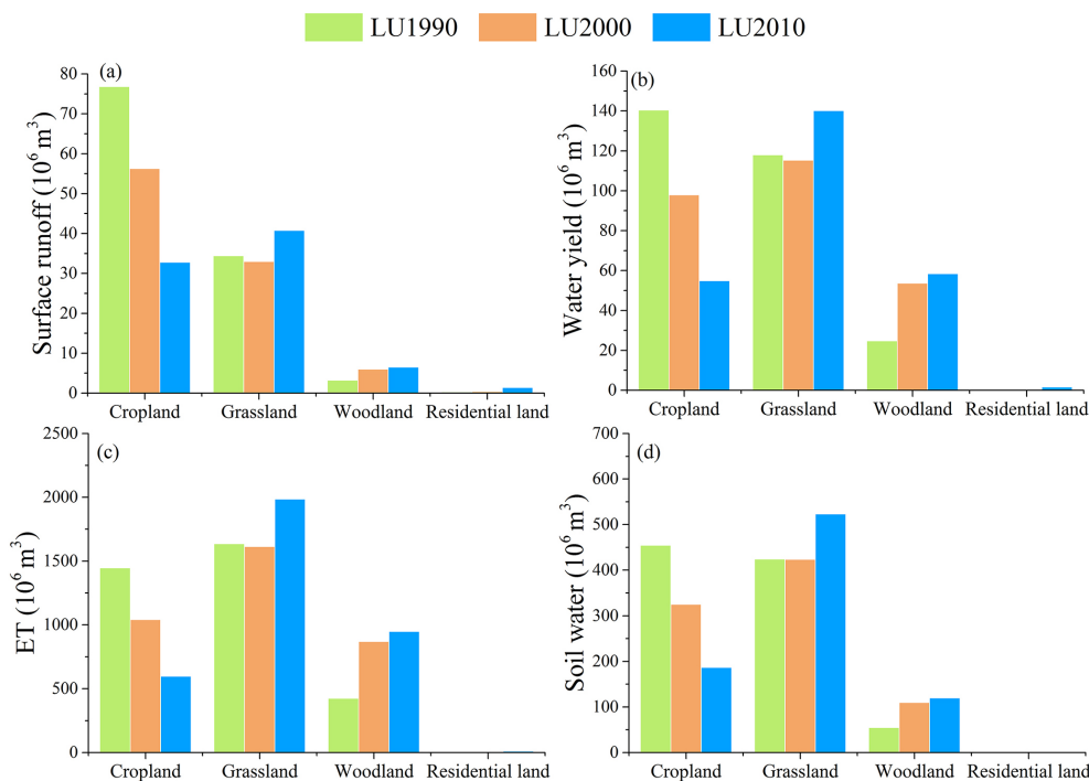
Figure 8. Calculated average annual total water volume under different land use scenarios.
