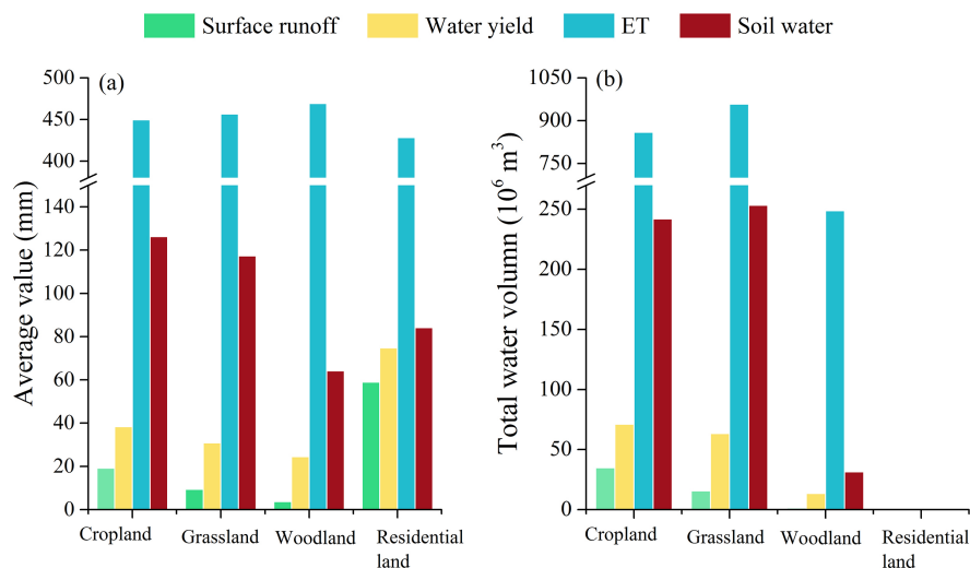
Figure 5. Calculated (a) unit area and (b) total annual hydrological components for the 18-year simulation period (1983–2000) for different land use types in the Yanhe Basin.
