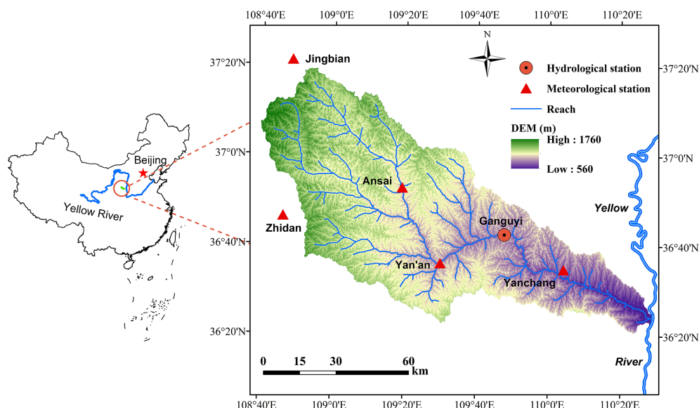
Figure 1. Map of the Yanhe Basin showing the elevation and the locations of the meteorological and hydrological stations.
