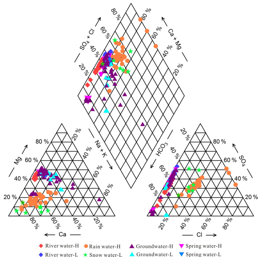
Figure 6. The piper diagram for groundwater, stream water, precipitation, and glacier and snow meltwater in the study area. “H” refers to high flows in the warm season; “L” refers to low flows in cold season.
