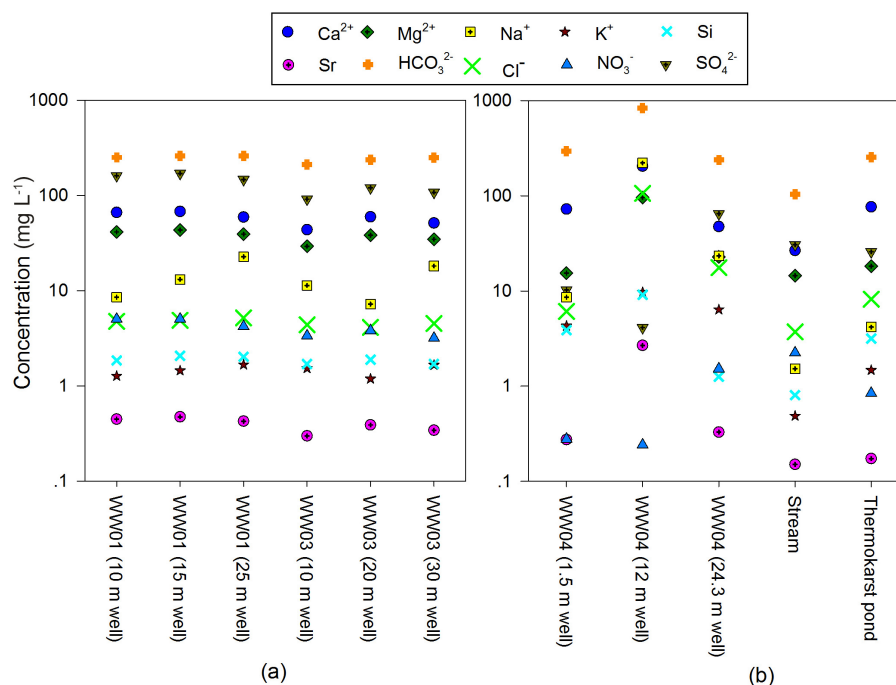
Figure 7. (a) Groundwater chemistry at different depths of the two clusters within the seasonal frost zone and (b) chemistry of groundwater, stream water and thermokarst pond water within the permafrost zone. WW01, WW03 and WW04 are symbols for clusters. The number in brackets means the specific screen depth of wells. Note the log scale on the y axis.
