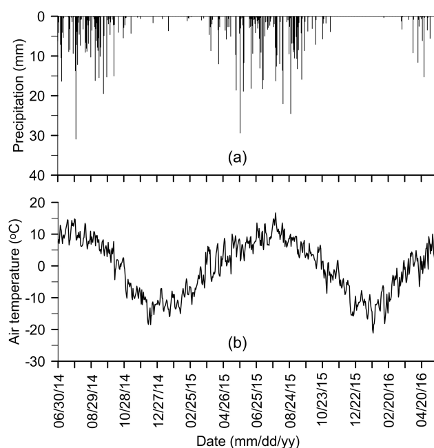
Figure 2. (a) Precipitation and (b) air temperature recorded at an elevation of 3649 m.a.s.l. within the Hulugou catchment from June 2014 to April 2016.
