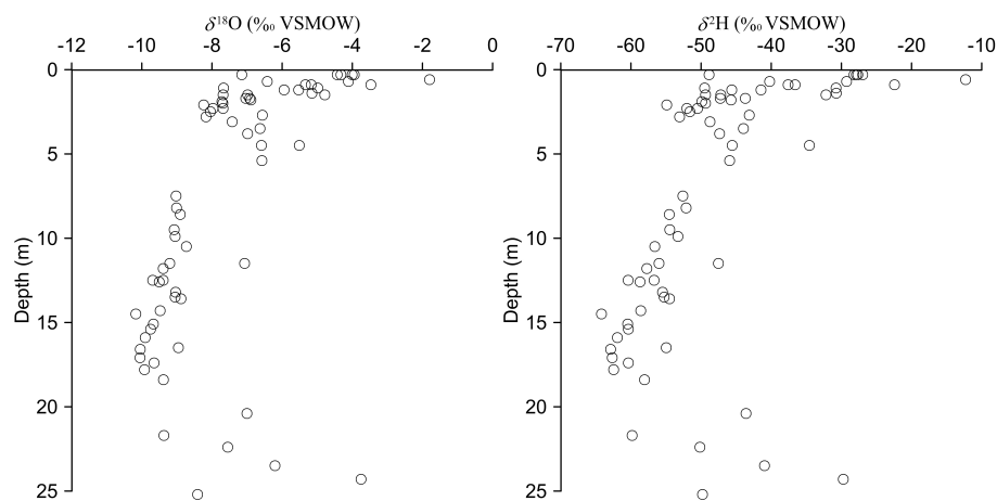
Figure 9. The variation of \delta^{18}\text{O} and \delta^2\text{H} in water and ice extracted from sediment cores with depth at cluster WW04.
