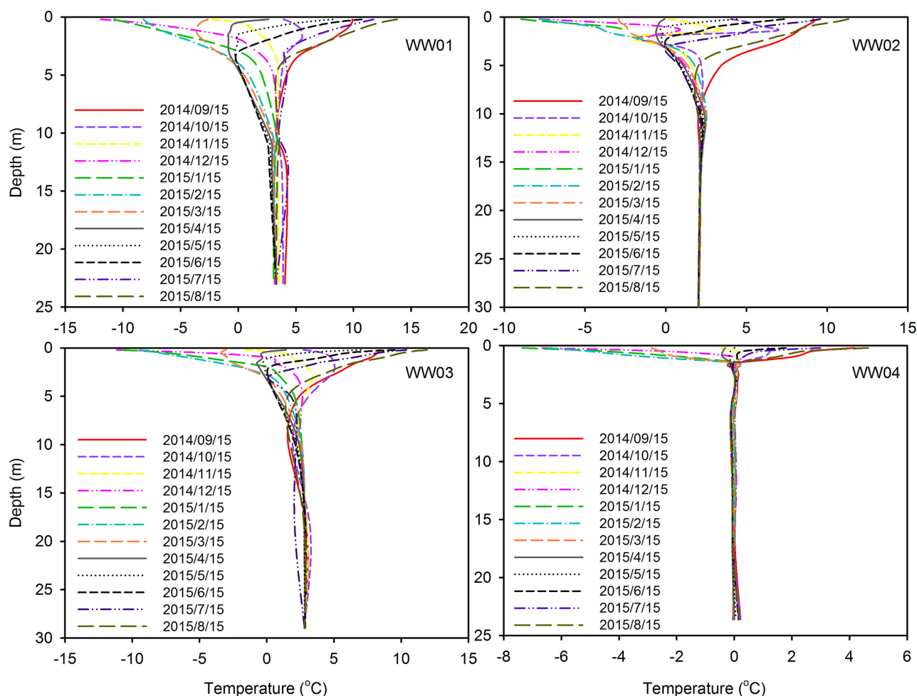
Figure 5. Temperature envelopes in the sediments at clusters WW01, WW02 and WW03 within the seasonal frost zone, as well as cluster WW04 within the permafrost zone.
