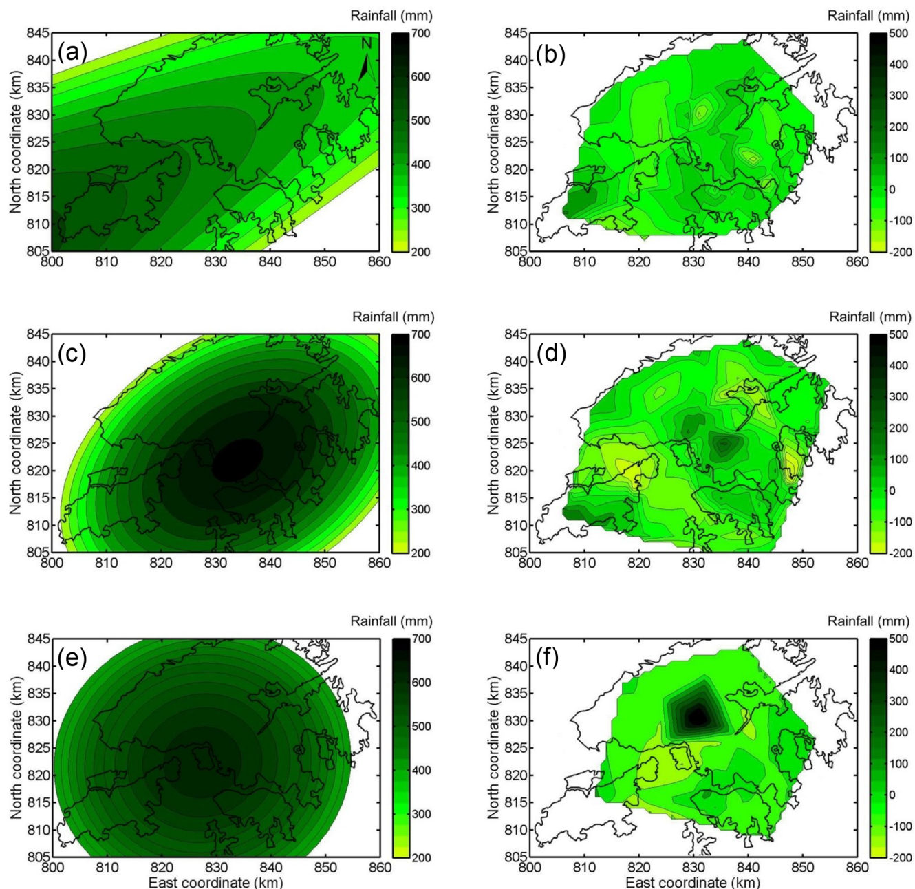
Figure 12. Trend surfaces and residuals of the total rainfall amounts: (a) and (b) show the 5–7 June 2008 storm; (c) and (d) show the 17–21 August 2005 storm; (e) and (f) show the 22–24 July 1994 storm.
