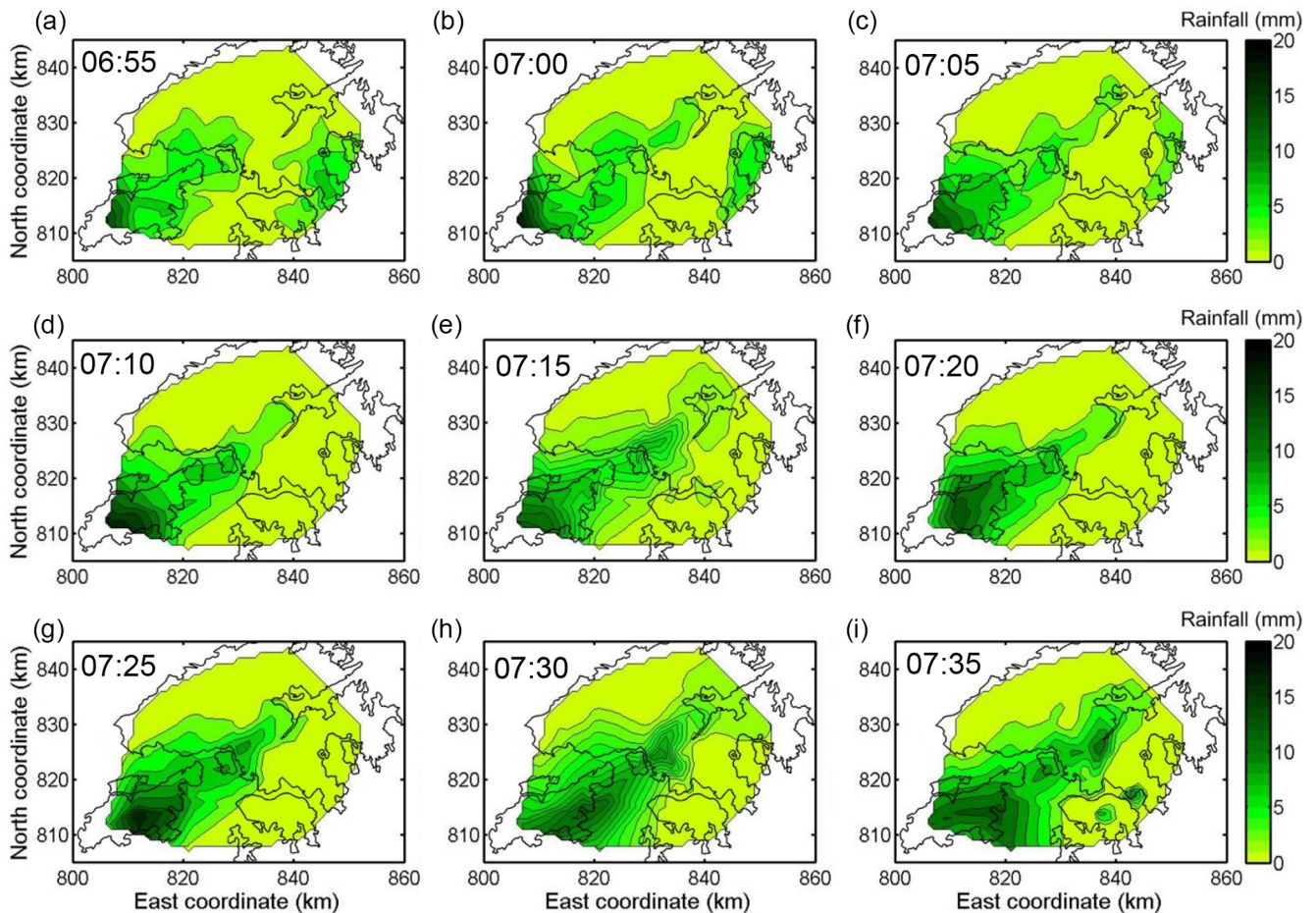
Figure 9. Instantaneous rainfall process from 06:55 to 07:35 LT on 7 June 2008.
