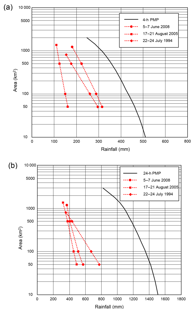
Figure 8. Magnitudes of the three storms characterized by (a) 4 h PMP and (b) 24 h PMP (modified from AECOM and Lin, 2015).
