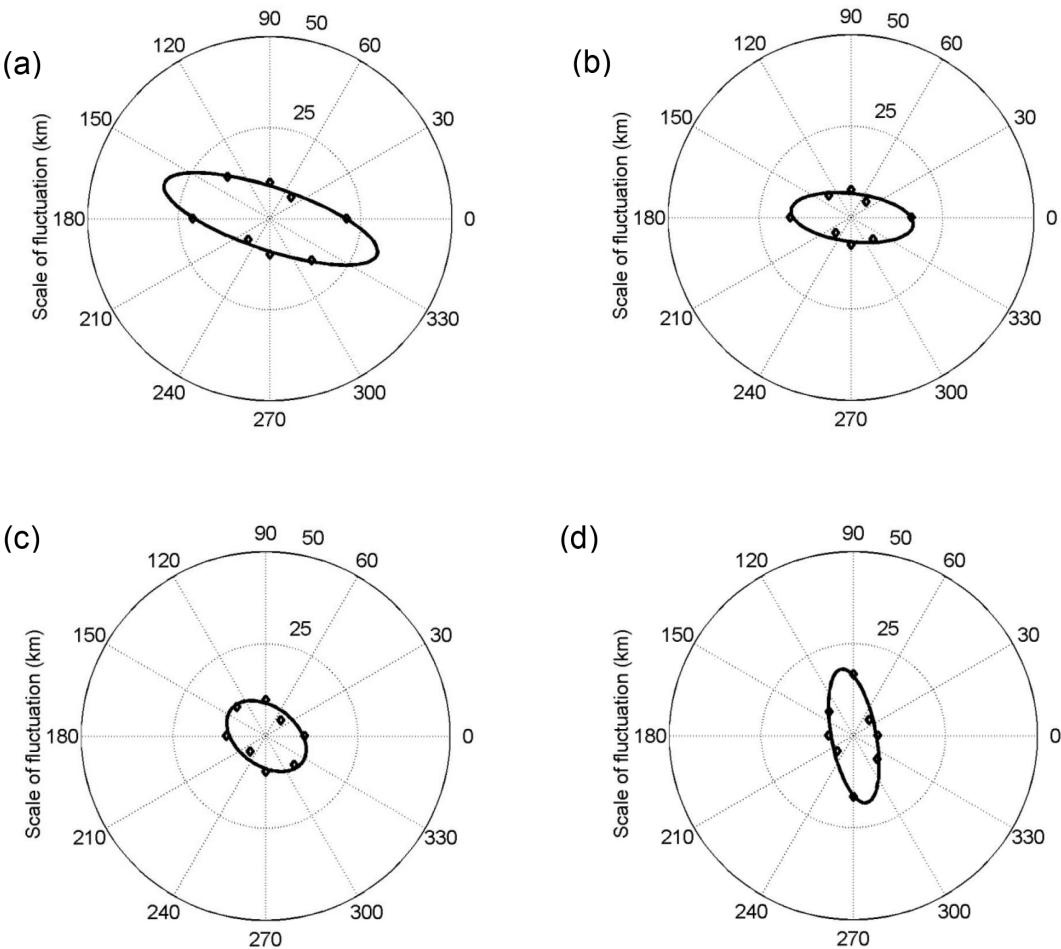
Figure 13. Scale of fluctuation values and ellipse-fitting curves for the 5–7 June 2008 storm: (a) maximum rolling 4 h rainfall, (b) maximum rolling 12 h rainfall, (c) maximum rolling 24 h rainfall, and (d) maximum rolling 36 h rainfall.
