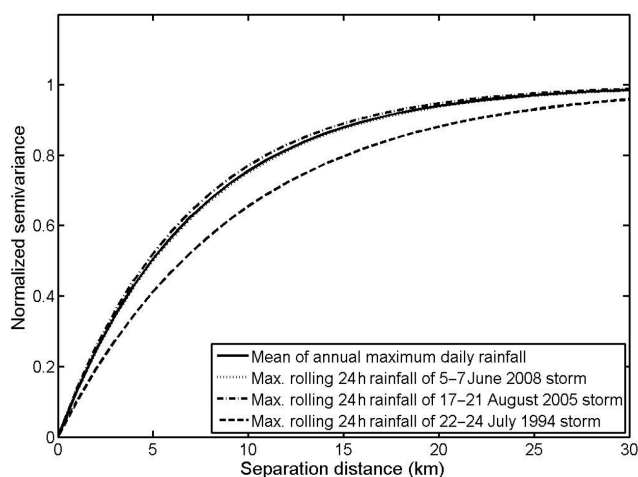
Figure 17. Normalized semivariances of the maximum rolling 24 h rainfall of the three storms and the mean annual maximum daily rainfall in Hong Kong.
