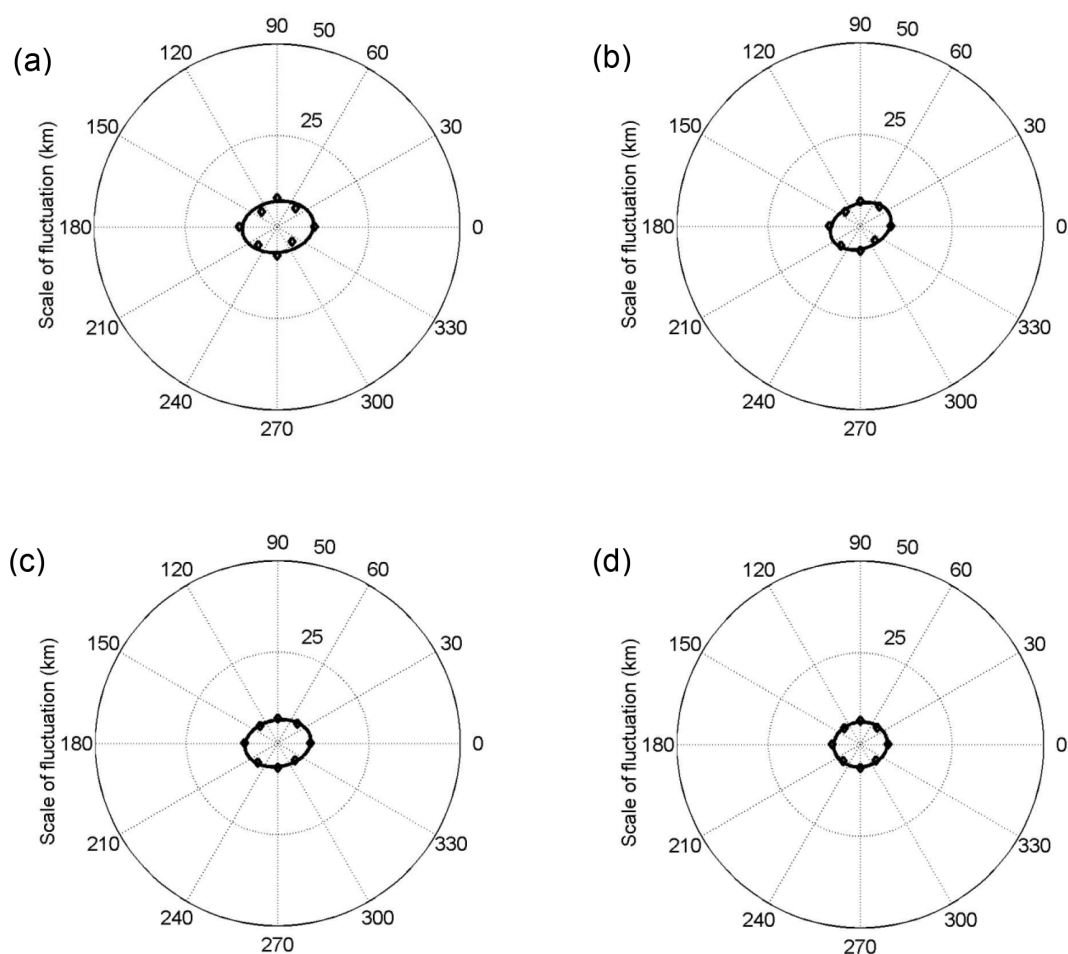
Figure 15. Scale of fluctuation values and ellipse-fitting curves for the 22–24 July 1994 storm: (a) maximum rolling 4 h rainfall, (b) maximum rolling 12 h rainfall, (c) maximum rolling 24 h rainfall, and (d) maximum rolling 36 h rainfall.
