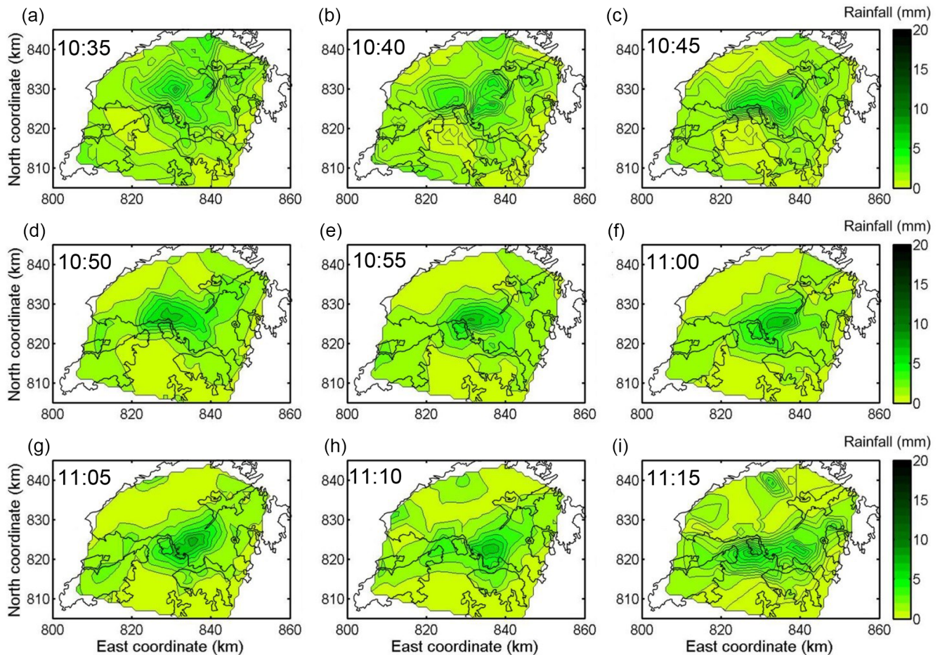
Figure 10. Instantaneous rainfall process from 10:35 to 11:15 LT on 20 August 2005.
