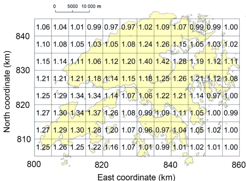
Figure 4. The 24 h orographic intensification factors in Hong Kong (modified from AECOM and Lin, 2015).
