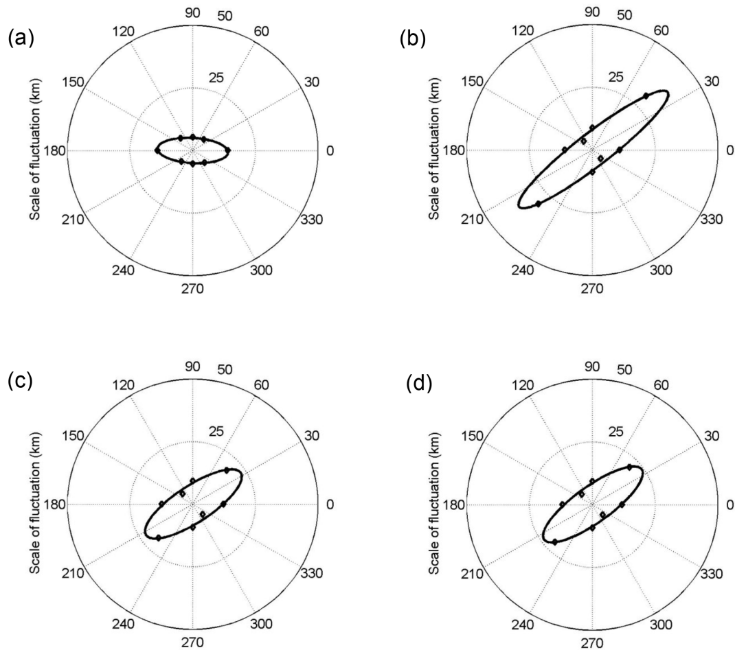
Figure 14. Scale of fluctuation values and ellipse-fitting curves for the 17–21 August 2005 storm: (a) maximum rolling 4 h rainfall, (b) maximum rolling 12 h rainfall, (c) maximum rolling 24 h rainfall, and (d) maximum rolling 36 h rainfall.
