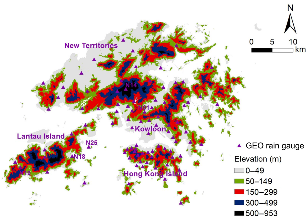
Figure 3. The GEO rain-gauge network in Hong Kong.
