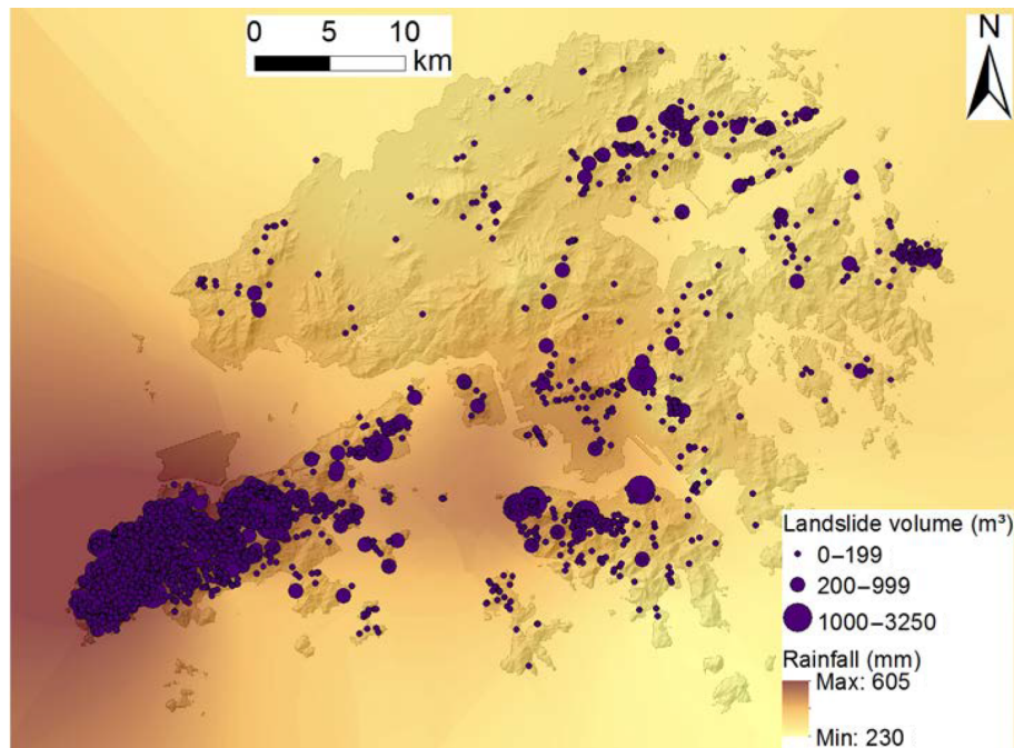
Figure 1. Spatial distributions of the maximum 24 h rolling rainfall and the landslides triggered in Hong Kong on 5–7 June 2008.
