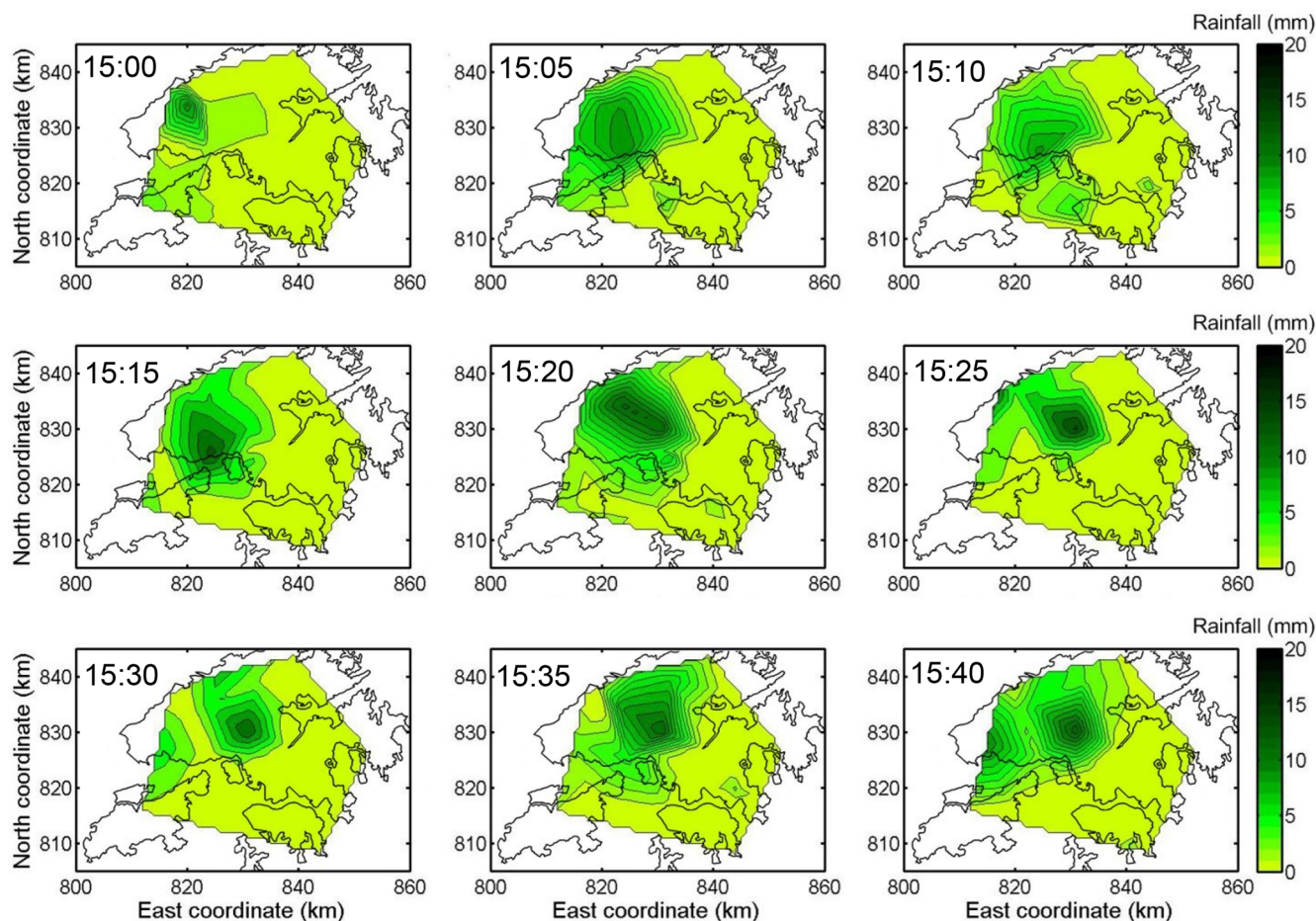
Figure 11. Instantaneous rainfall process from 15:00 to 15:40 LT on 23 July 1994.
