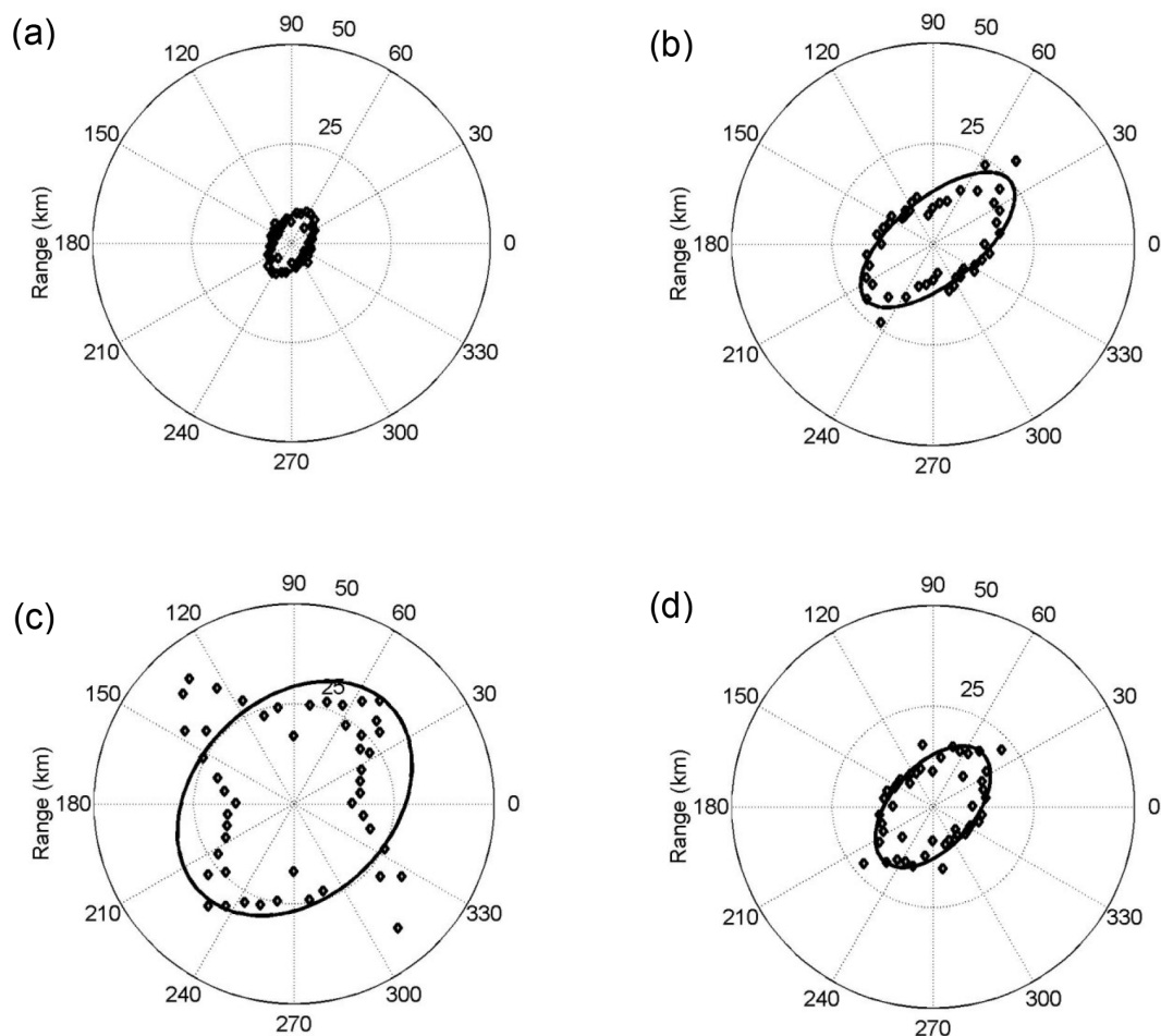
Figure 16. Range values for (a) the 18 May 2007 storm (16:30 LT), (b) the 19 May 2007 storm (16:00 LT), (c) the 19 April 2008 storm (20:00 LT), and (d) the 15 September 2009 storm (15:00 LT; modified from Liu, 2013).
