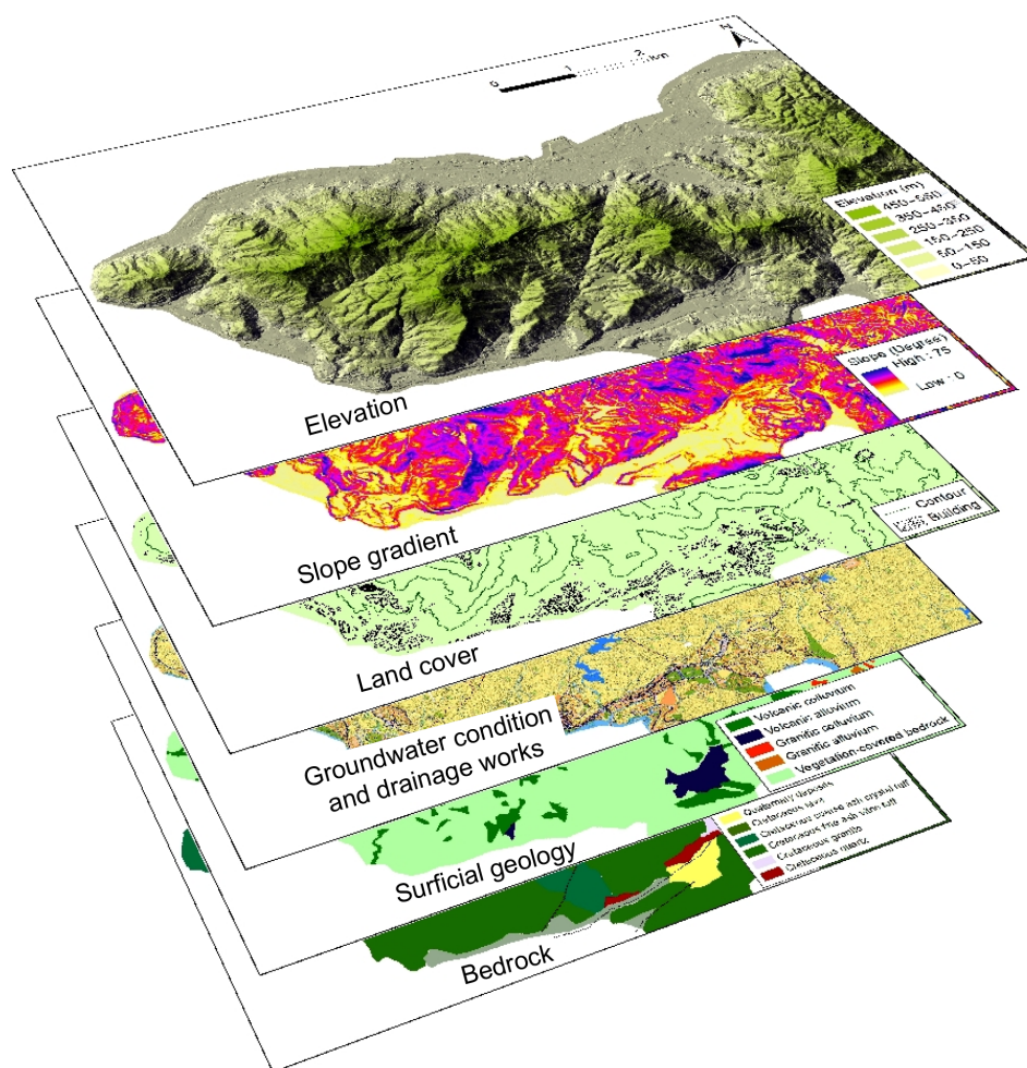
Figure 2. Geotechnical and environmental factors that affect the triggering of natural terrain landslides.
