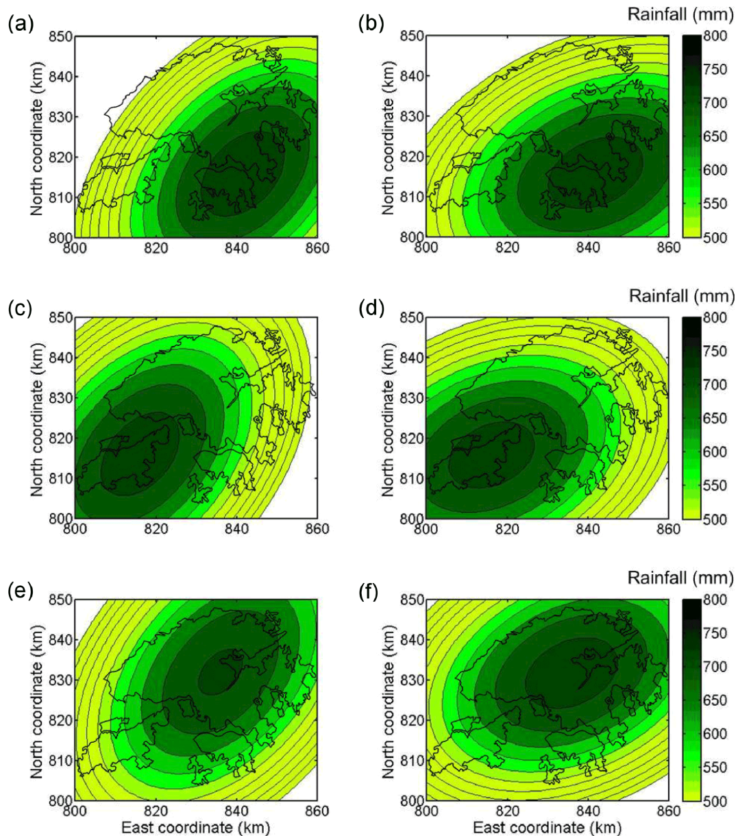
Figure 5. Trend surfaces of 24 h PMP with (a) NE–SW orientation 45^\circ ; (b) ENE–WSW orientation 22.5^\circ centered at Hong Kong Island; (c) NE–SW orientation 45^\circ ; (d) ENE–WSW orientation 22.5^\circ centred at Lantau Island; (e) NE–SW orientation 45^\circ ; and (f) ENE–WSW orientation 22.5^\circ centred at Tai Mo Shan (modified from AECOM and Lin, 2015).
