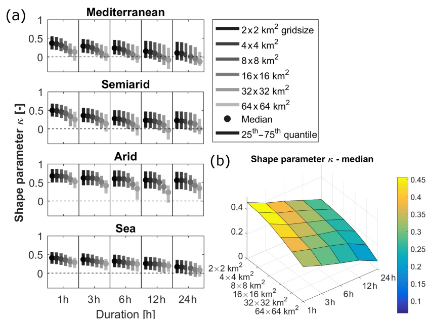
Figure 3. (a) Distribution (median and 25–75th quantiles) of the shape parameter derived aggregating radar estimates on grid sizes increasing from 2 km × 2 km to 64 km × 64 km. (b) Median of the shape parameters (all climates) derived aggregating radar estimates as a function of the spatial and of the temporal aggregation scales
