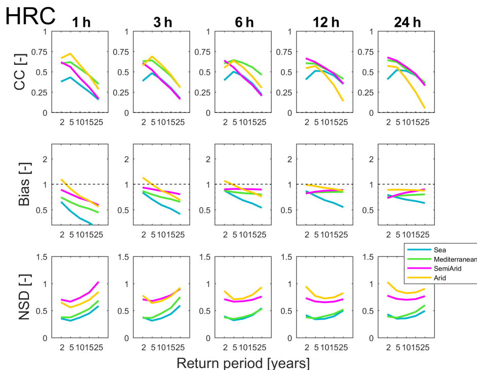
Figure 7. Comparison of IDF values between HRC and radar for different climatic regions. Blue lines represent sea areas while green, pink, and orange lines represent the Mediterranean, semiarid, and arid climates respectively. The upper row of panels shows the CC for different durations, the middle row the bias, and the lower row the NSD.
