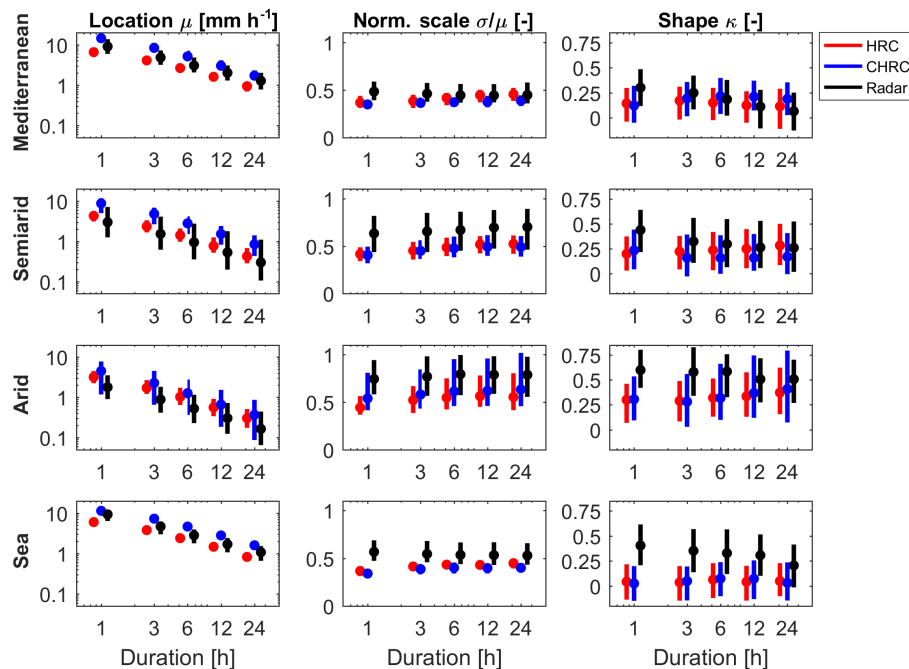
Figure 2. Distribution (median and 25–75th quantiles) of the GEV parameters derived from satellite (HRC and CHRC) and radar datasets. Note that scale parameters are normalized over the corresponding location parameters. The parameters for different products are represented around the corresponding duration; therefore, the logarithmic scale in the x axes should be interpreted accordingly.
