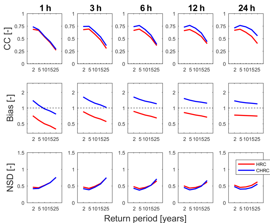
Figure 6. Comparison of IDF values between HRC and radar (red) and CHRC and radar (blue). The upper row of panels shows the CC for different durations, the middle row the bias and the lower row the NSD.
