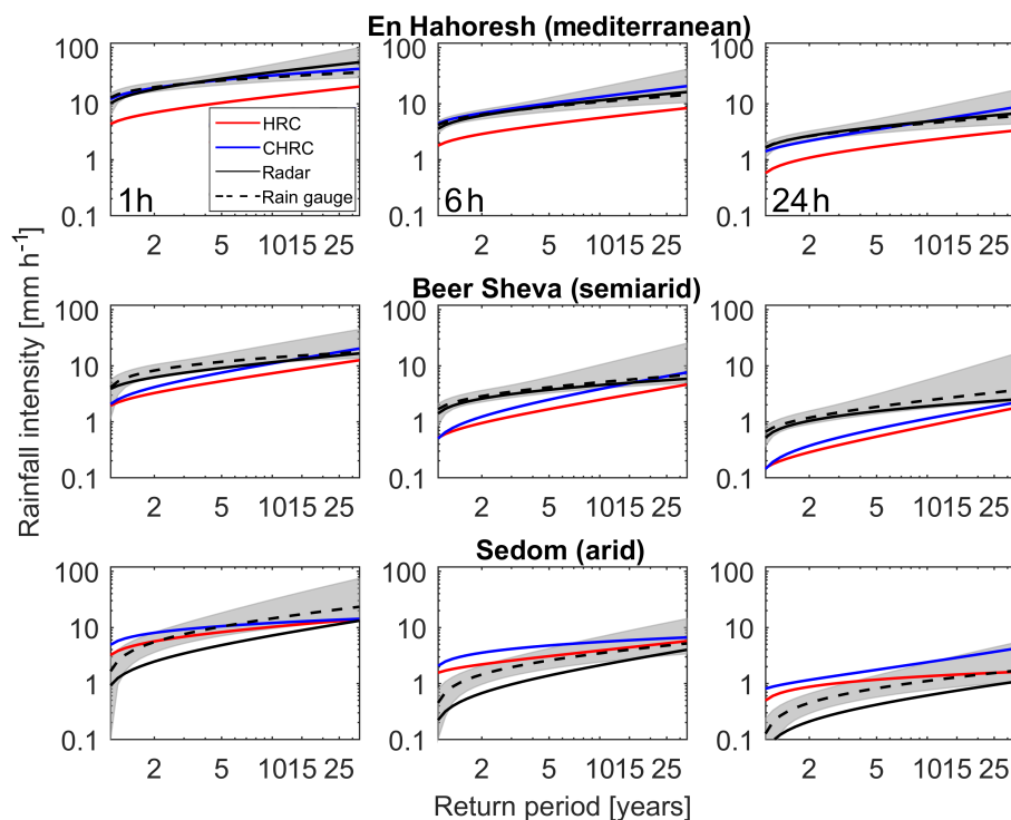
Figure 4. Visual comparison of the annual maxima and of the IDF curves derived for the examined 16 years (1998–2013) from HRC (red), CHRC (blue), radar (solid black), and rain gauge (dashed black). The shaded area represents the 95 % confidence interval of the rain gauge IDF. Three example locations in the Mediterranean (En Hahores), semiarid (Beer Sheva) and arid (Sedom) climates and for 1, 6, and 24 h durations are shown (see gauge location in Fig. 1).
