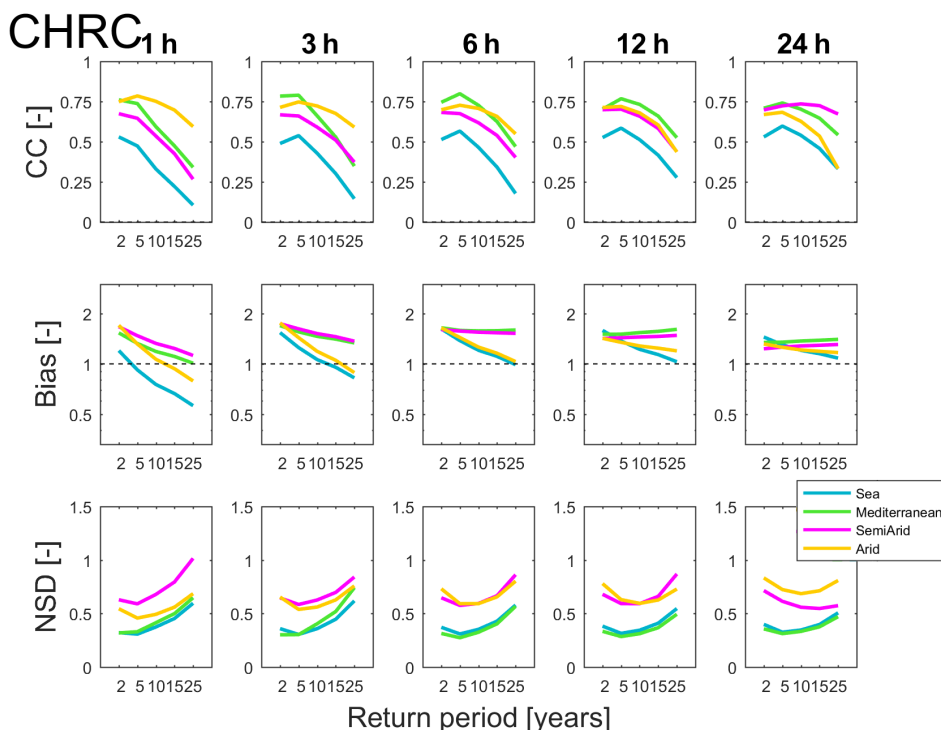
Figure 8. Comparison of IDF values between CHRC and radar for different climatic regions. Blue lines represent sea areas while green, pink, and orange lines represent the Mediterranean, semiarid, and arid climates respectively. The upper row of panels shows the CC for different durations, the middle row the bias, and the lower row the NSD.
