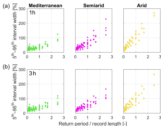
Figure 10. Relative uncertainty (width of the 5–95th quantile interval of the 999 bootstrap sampling repetitions normalized over the rain gauge-IDF value) plotted against the ratio between the estimated return period and the record length. The first row of panels shows the results for 1 h duration, the second row for 3 h. Columns of panels show results for each climatic region.
