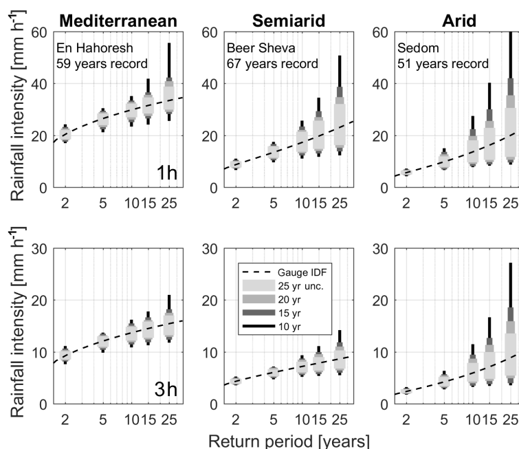
Figure 9. Uncertainty related to the record length for 1 and 3 h durations for three example cases in the Mediterranean (En Hahores), semiarid (Beer Sheva) and arid (Sedom) climates. The dashed lines show the IDF curves from the full records (59, 67, and 51 years, respectively) and the vertical bars show the width of the 5–95th quantile interval of the 999 bootstrap sampling repetitions for record lengths of 10, 15, 20, and 25 years. Width and light of the colour of the bars increase with the record length.
