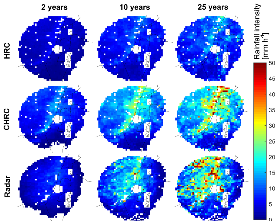
Figure 5. Example of IDF maps for 3 h duration from HRC, CHRC, and radar for 2-, 10-, and 25-year return periods. Only the pixels included in the analyses are shown.
