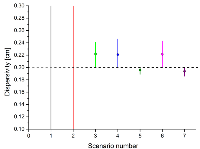
Figure 14. Posterior mean values and 95 % confidence intervals of the dispersivity for the different scenarios.
