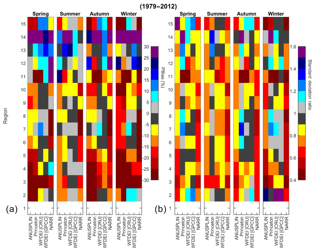
Figure 6. Portrait diagram showing the accuracy ( P_{Bias} ) (a) and amplitude of the variations ( \sigma_G/\sigma_R ) (b) of each type of gridded precipitation products when evaluating against the precipitation-gauge station data in each ecozone (regions 1 to 15) in four seasons for the time period of 1979 to 2012. Each column indicates one gridded precipitation product and each row represents one ecozone with numerical code corresponding to region shown in Fig. 1. White indicates that no data are available due to no precipitation-gauge stations existing in that region.
