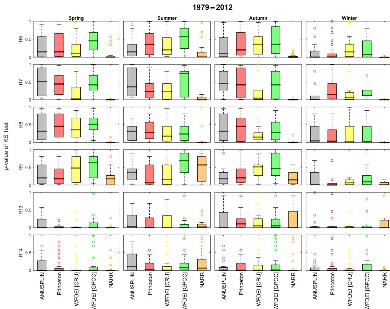
Figure 3. Distributions of p value of the K–S test in four seasons for the period of 1979 to 2012 (long-term comparison without CaPA). Note that the numbers of precipitation-gauge stations in each ecozone are different (see Table 4). The p values of regions 6 to 9, and 13 to 14 (R6–R9 and R13–R14), which are more than or equal to 10 stations, were only shown for illustration in box-and-whisker plots with bottom, band (black thick line), and top of the box indicating the 25th, 50th (median), and 75th percentiles respectively.
