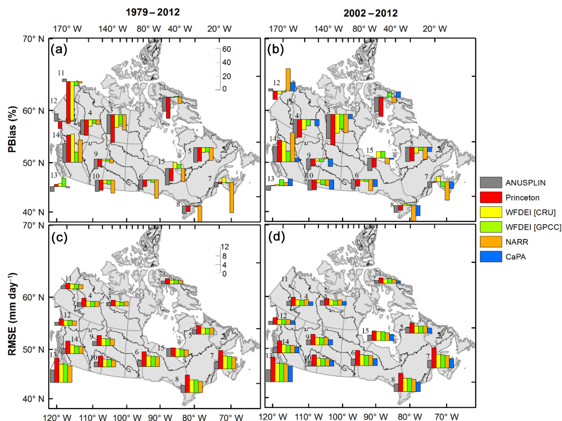
Figure 9. Bar graphs showing the annual accuracy ( P_{\text{Bias}} ) (first row) and magnitude of the errors (RMSE) (second row) of each precipitation dataset for the period of 1979 to 2012 (a, c) and 2002 to 2012 (b, d) in different ecozones. The white bar shows the scale of the bars with the number beside it indicating the value of the bar.
