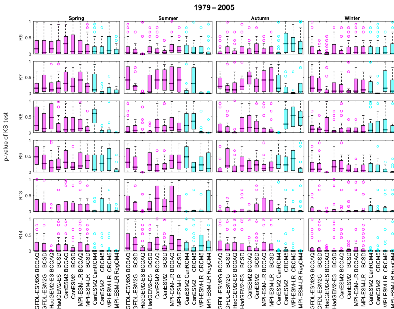
Figure 5. Distributions of p value of the K–S test in four seasons for the period of 1979 to 2005 (long-term comparison of PCIC and NA-CORDEX). Note that the numbers of precipitation-gauge stations in each ecozone are different (see Table 4). The p values of regions 6 to 9, and 13 to 14 (R6–R9, and R13–R14), which are more than or equal to 10 stations, were only shown for illustration in box-and-whisker plots with bottom, band (black thick line), and top of the box indicating the 25th, 50th (median), and 75th percentiles respectively.
