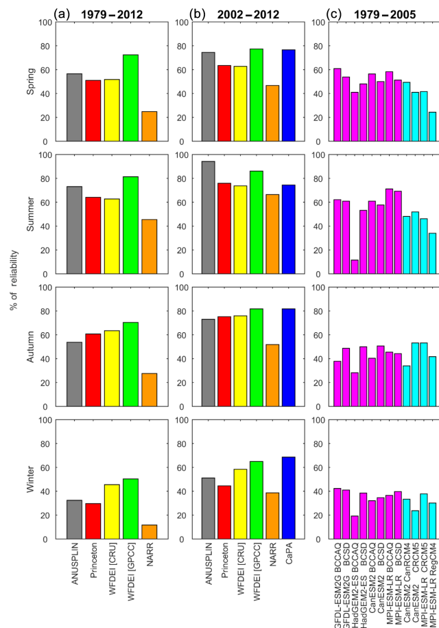
Figure 2. The percentage of reliability, calculated by Eq. (1), of each precipitation dataset in four seasons for the period of 1979 to 2012 (a), 2002 to 2012 (b), and 1979 to 2005 (c) across Canada. The higher the percentage, the more reliable the precipitation dataset. Different colours represent different precipitation products, with magenta representing the whole PCIC datasets and cyan representing the whole NA-CORDEX datasets. The full names of the precipitation products are provided in Tables 1, 2, and 3.
