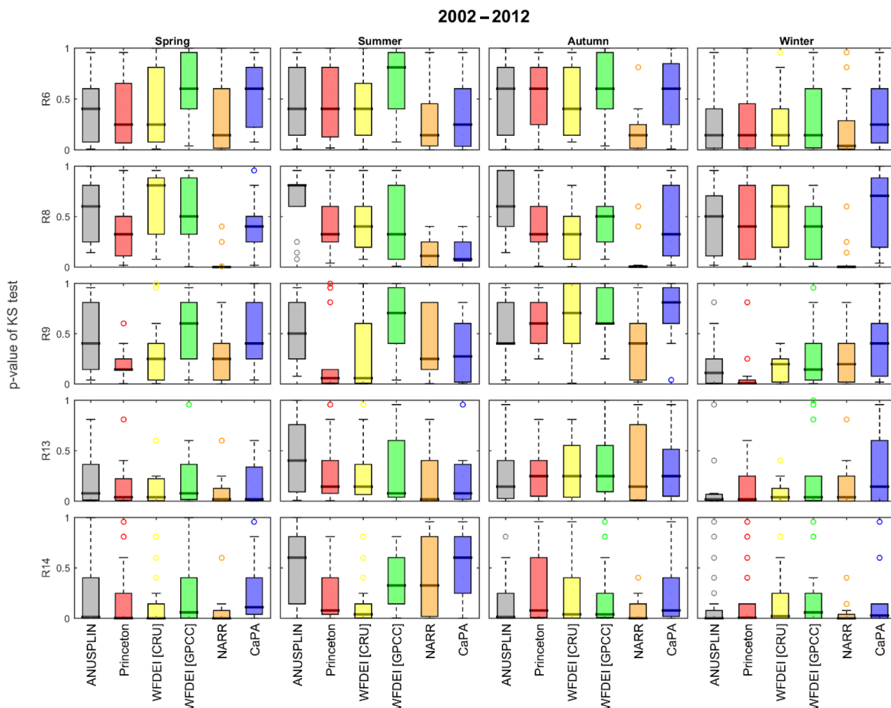
Figure 4. Distributions of p value of the K–S test in four seasons for the period of 2002 to 2012 (short-term comparison with the inclusion of CaPA). Note that the numbers of precipitation-gauge stations in each ecozone are different (see Table 4). The p values of regions 6, 8 to 9, and 13 to 14 (R6, R8–R9, and R13–R14), which are more than or equal to 10 stations, were only shown for illustration in box-and-whisker plots with bottom, band (black thick line), and top of the box indicating the 25th, 50th (median), and 75th percentiles respectively.
