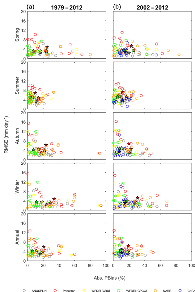
Figure 8. Scatter plots showing absolute P_{\text{Bias}} ( x axis) versus RMSE ( y axis) of each precipitation dataset in four seasons and the entire year for the period of 1979 to 2012 (a) and 2002 to 2012 (b). Each hollow circle represents one ecozone and the solid stars indicate the overall average across ecozones.
