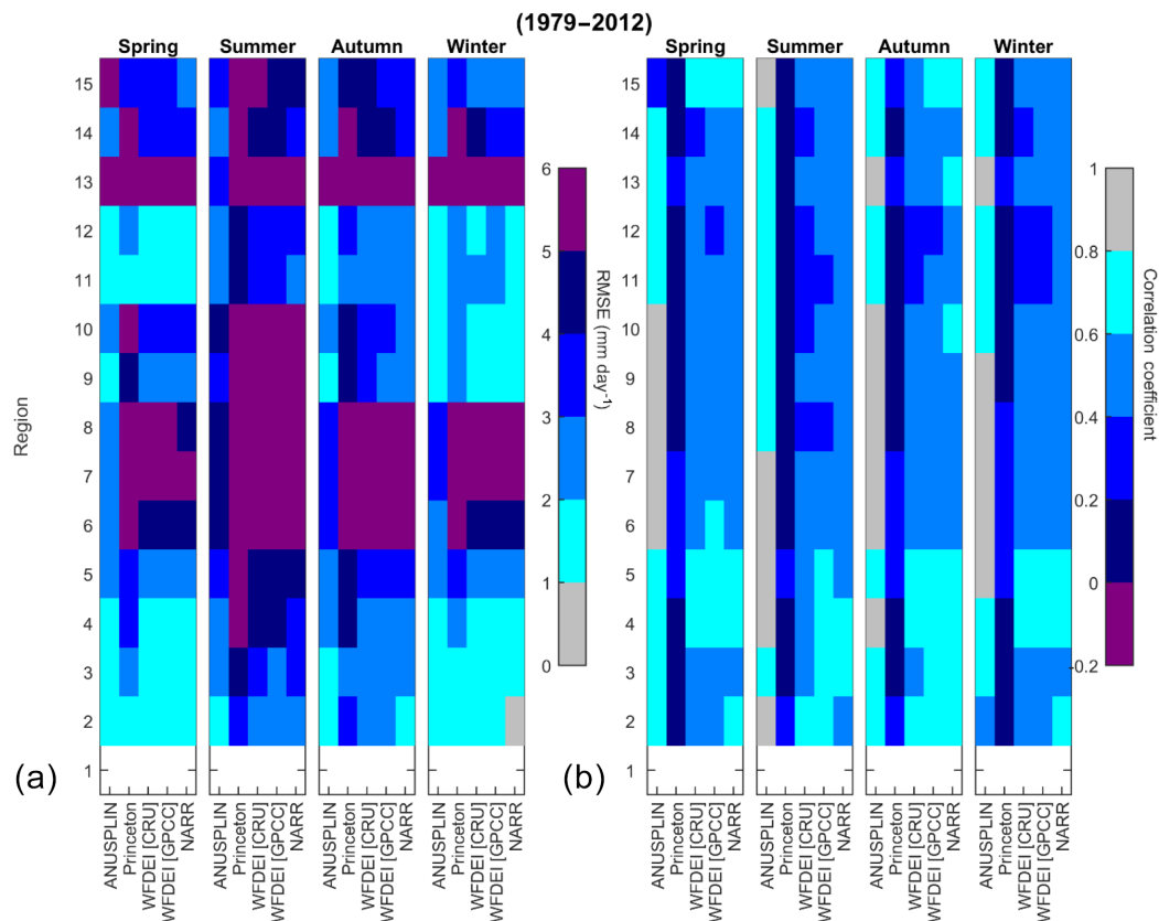
Figure 7. Portrait diagram showing magnitude of the errors (RMSE) (a), and strength and direction of relationship between gridded products and precipitation-gauge stations ( r ) (b) of each type of gridded precipitation product when evaluating against the precipitation-gauge station data in each ecozone (regions 1 to 15) in four seasons for the time period of 1979 to 2012. Each column indicates one gridded precipitation product and each row represents one ecozone with numerical code corresponding to the region shown in Fig. 1. White indicates that no data are available due to no precipitation-gauge stations existing in that region.
