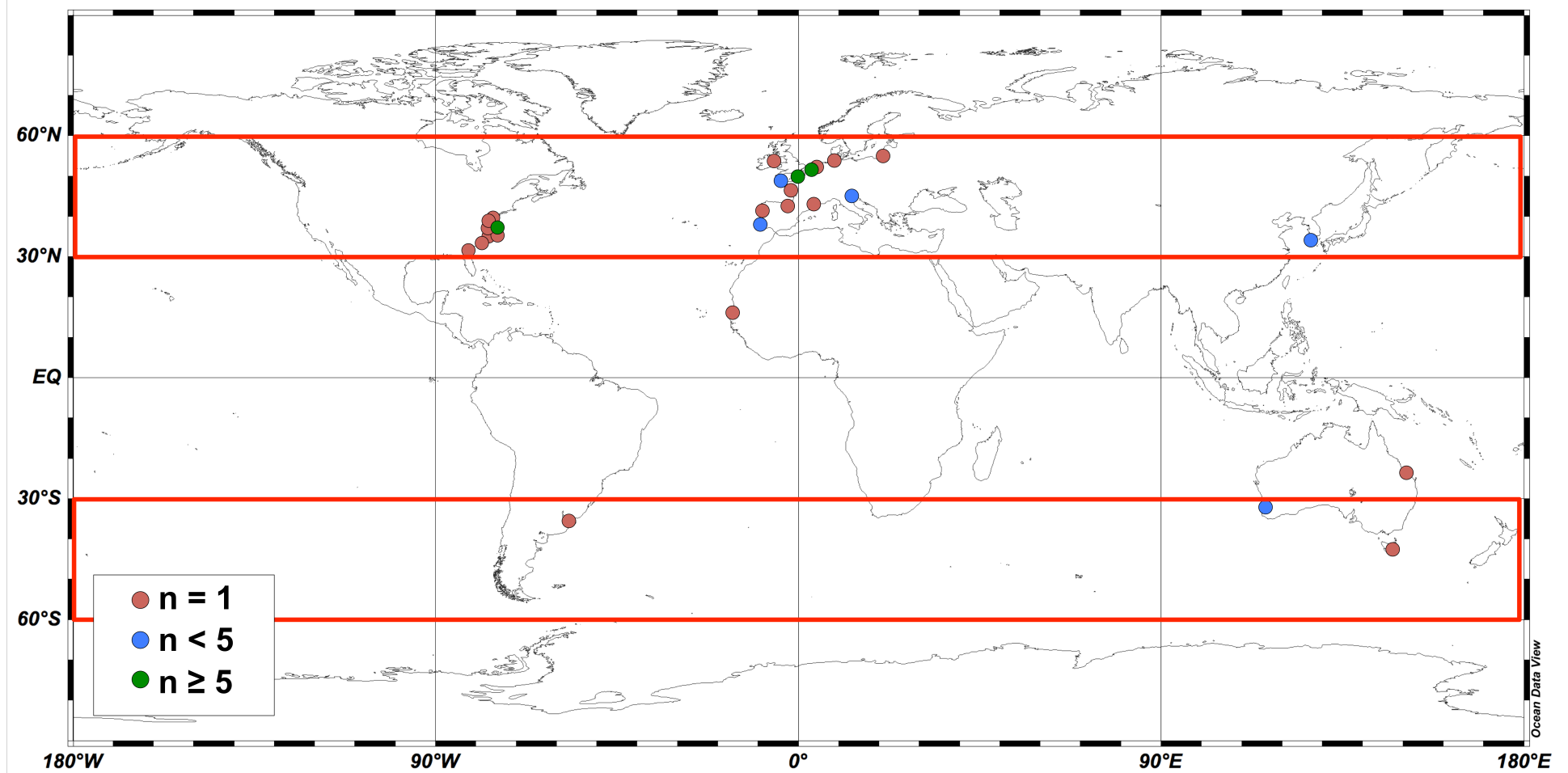
Location of published estuarine biogeochemical model applications ( n=51 ) and their distribution amongst different climatic zones. Red, blue and green dots correspond to locations in which 1, and less than 5 or more than 5 model applications have been published, respectively. The limits of the temperate zones ( 30^\circ < \text{lat} < 60^\circ ) in either hemisphere are highlighted in red.
