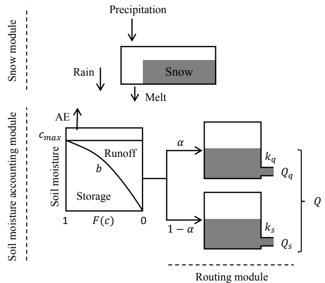
Figure A1. Schematic representation of the rainfall-runoff conceptual model structure used.
