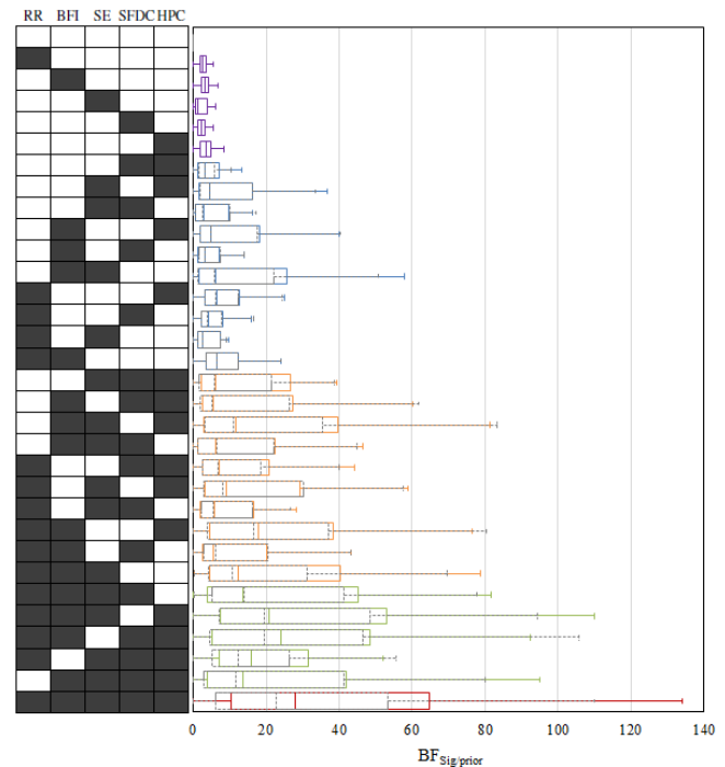
Figure 3. Boxplots representing the distribution of the Bayes factor for each combination of signatures for synthetic streamflow data. The colored boxplots correspond to the results obtained when inter-signature error correlations are considered in the likelihood function, whereas the grey dashed boxplots correspond to the results obtained assuming that the inter-signature errors are independent.
