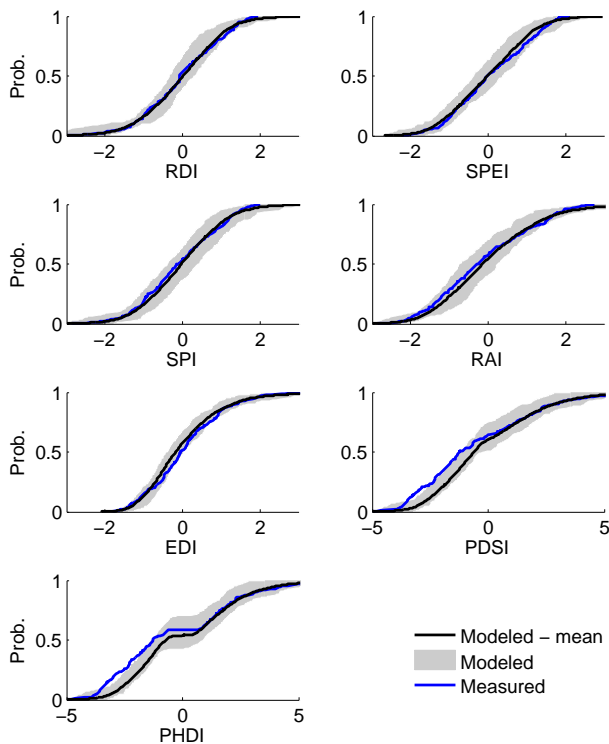
Figure 4. Empirical cumulative distribution functions of daily precipitation for present and future climate scenarios.
