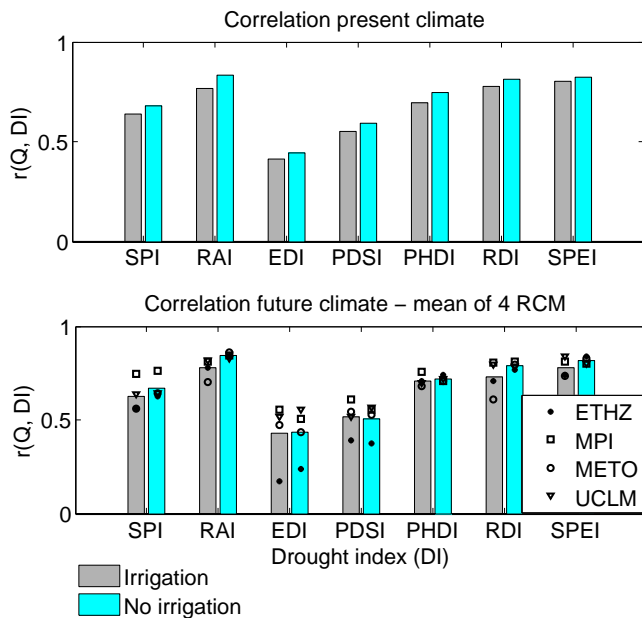
Figure 5. Correlation coefficient r between the drought indices and discharge. The irrigation scenarios are PIRR in the present climate and FUTIRR in the future climate. In the future climate (bottom panel), the plotted bars are the average of the outputs of the four regional climate models. See Table 2 for information about the four regional climate models.
