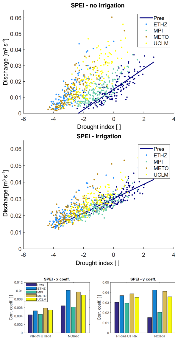
Figure 6. Performance of SPEI in future climate for annual discharge. The blue line is the linear regression between SPEI and discharge in present climate. Top panel: NOIRR scenario, large model bias. Second panel: FUTIRR scenario, no significant model bias. Bottom panel: the two coefficients of the linear regression between Q and SPEI in each climate.
