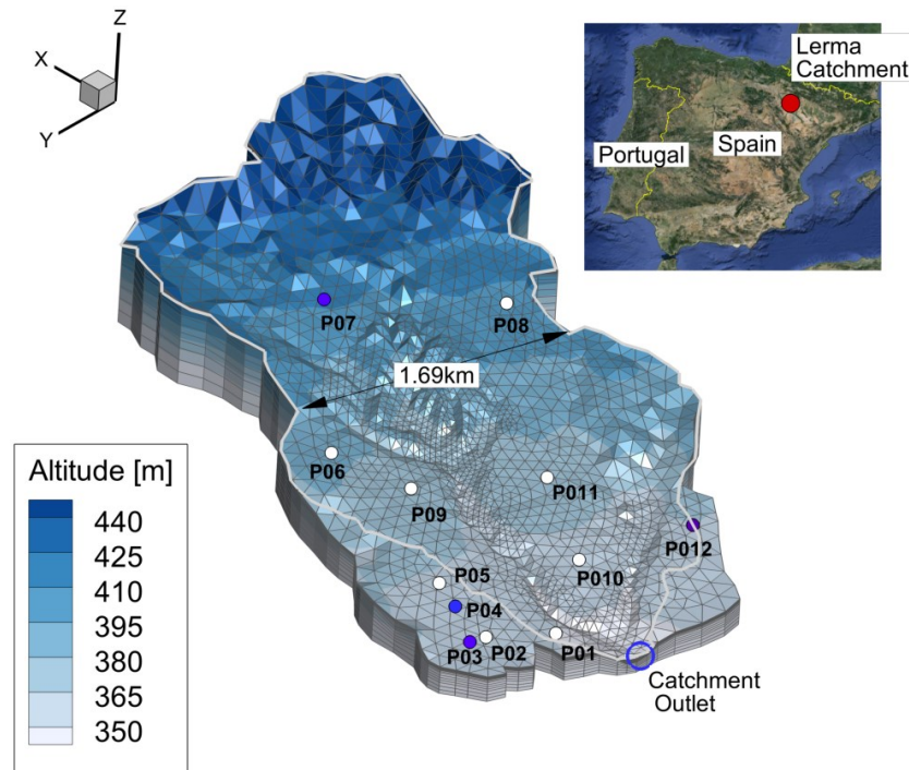
Figure 1. Surface elevation of the Lerma catchment (m a.s.l.). The observation wells drilled in 2010 are indicated by blue circles and the ones drilled in 2008 are indicated by white circles. The gray line represents the limits of the surface flow domain. Vertical exaggeration: 5 : 1. Modified from von Gunten et al. (2014, 2015).
