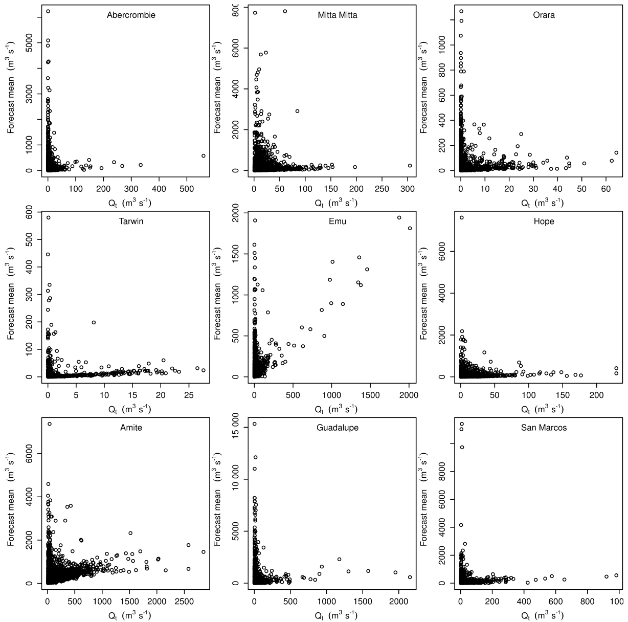
Figure 7. Comparison of streamflow observations with the streamflow forecast mean for each catchment when the residual distribution is fitted by a Student's t distribution.
