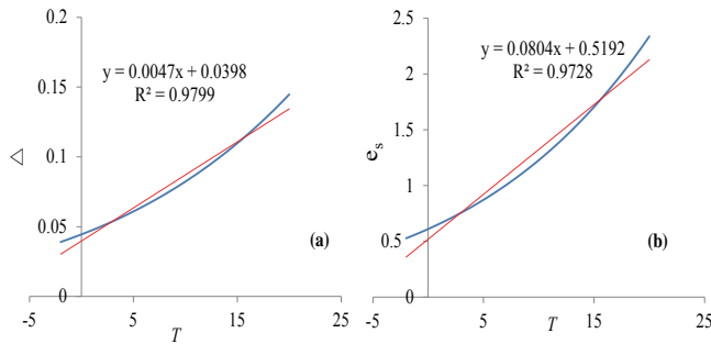
Figure A1. The relationship of (a) ( \text{kPa } ^\circ\text{C}^{-1} ) and (b) e_s (kPa) with temperature T ( ^\circ\text{C} ) change. The blue curves are the relationship of \Delta and e_s with T , respectively; the pink curves show the linear slope of \Delta and e_s with T ( T ranging from -2 to 20 ^\circ\text{C} ), respectively.
