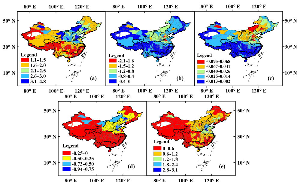
Figure 4. (a) Precipitation elasticity \varepsilon_P , (b) net radiation elasticity \varepsilon_{Rn} , (c) air temperature elasticity \varepsilon_T (unit: ^{\circ}\text{C} ), (d) wind speed elasticity \varepsilon_{U2} , and (e) relative humidity elasticity \varepsilon_{RH} of runoff in the 207 catchments.
