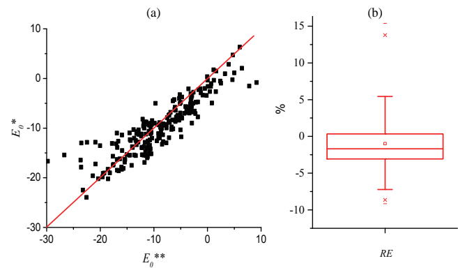
Figure 2. (a) Comparison between the potential evaporation change evaluated by Eq. (9), denoted as E_0^* (%), and that evaluated by Eq. (17), denoted as E_0^{**} (%), from 1961 to 2010, and (b) the relative error (RE) (%) caused by the first-order approximation, where RE = (E_0^* - E_0^{**}) / E_0^{**} , E_0^* , and E_0^{**} were the potential evaporation changes evaluated by Eqs. (9) and (17), respectively.
