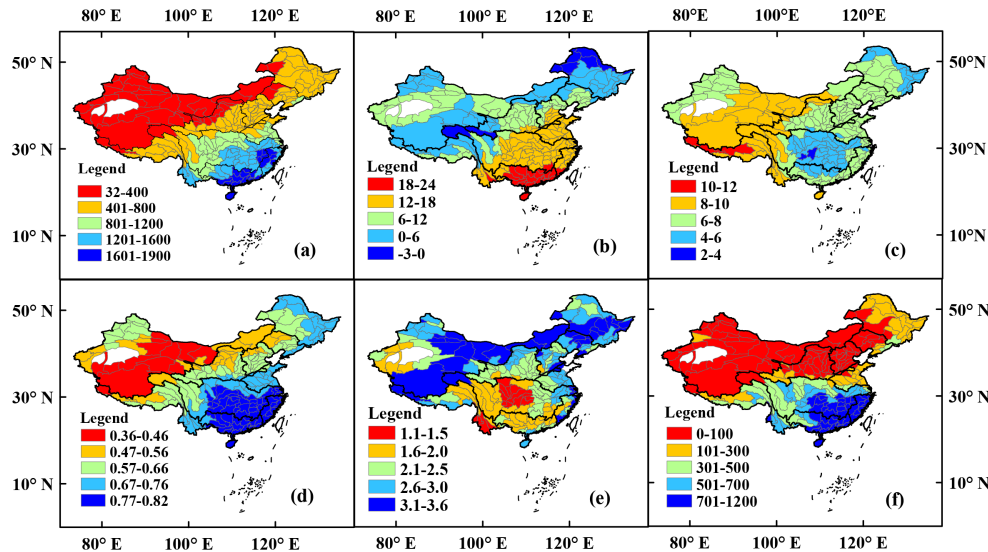
Figure 3. The mean annual (a) precipitation (unit: mm), (b) air temperature (unit: °C), (c) net radiation (unit: MJ m −2 d −1 ), (d) relative humidity, (e) wind speed at 2 m height (unit: m s −1 ), and (f) runoff (unit: mm) in the 207 catchments from 1961 to 2010.
