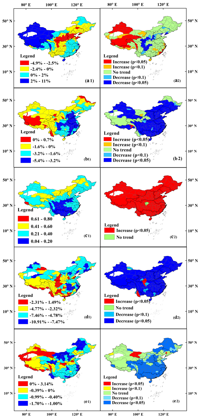
Figure 5. The changing trends for (a1) precipitation (unit: decade -1 ), (b1) net radiation (unit: decade -1 ), (c1) air temperature (unit: °C decade -1 ), (d1) wind speed (unit: decade -1 ), (e1) relative humidity (unit: decade -1 ); and the significance of the trends for (a2) precipitation, (b2) net radiation, (c2) air temperature, (d2) wind speed, (e2) relative humidity to runoff in the 207 catchments from 1961 to 2010.
