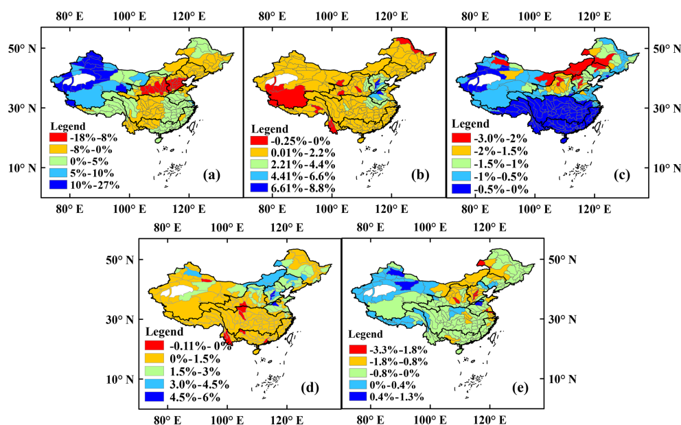
Figure 6. The contribution of (a) precipitation, (b) net radiation, (c) air temperature, (d) wind speed, and (e) relative humidity to runoff change in the 207 catchments from 1961 to 2010 (unit: decade).
