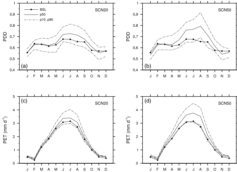
Figure 6. Projected and baseline (BSL) statistics for dry day probability (PDD) and mean daily PET for SCN20 and SCN50 for Thames catchment. For the ensemble projections the central estimate (p50) and upper and lower estimates represented by the 90th (p90) and 10th (p10) percentiles are shown.
