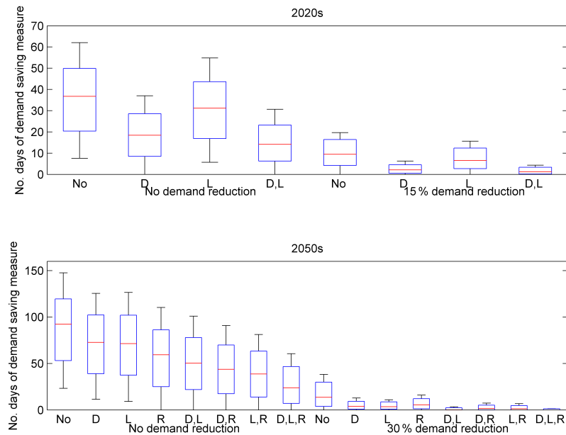
Figure 10. Number of DS4 days per 100 years for SCN20 and SCN50 under climate and population projections, given a range of supply and demand management options. No = no supply measures; D = desalination plant providing up to 150 ML day -1 ; L = leakage targets (24.2 % by 2020; 18.5 % by 2050); R = reservoir of 100 million m 3 . Results are presented with no reduction in per capita demand and 15 % reduction in 2020 and 30 % reduction in 2050. Box plots indicate the median, 25th, and 75th percentile values; whiskers show the 10th and 90th percentile values.
