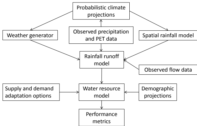
Figure 1. Methodological approach for the study of current and future water resources for the Thames.
