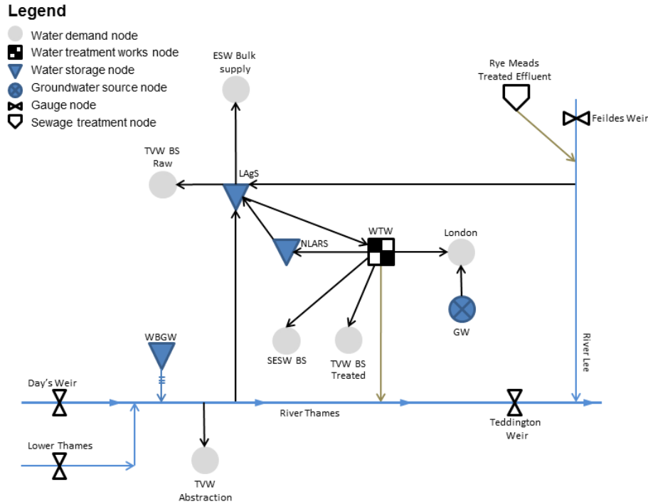
Figure 4. A schematic of LARaWaRM indicating the various water resource system components and interactions. (NB: groundwater is included as an aggregate inflow of 467.4 ML day -1 to meet London’s demand. A proportion of the inflow to the water treatment works is leakage; this is equivalent to 12 % of demand and is returned back to the river and modelled as a contribution to the minimum environmental flow.)
