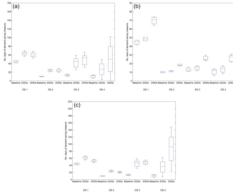
Figure 8. Number of demand saving days per 100 years (DS1–DS4) under BSL, SCN20, and SCN50 scenarios for (a) climate change projections only; (b) population growth projections only; (c) both climate and population projections, in all cases per capita demand remains constant at present-day value. Box plots indicate the median, 25th, and 75th percentile values; whiskers show the 10th and 90th percentile values.
