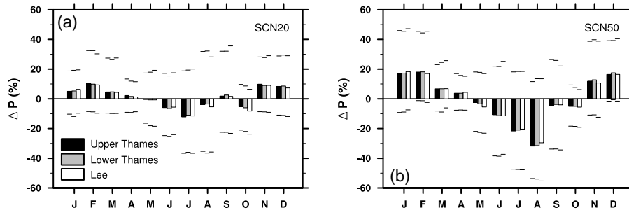
Figure 5. Percentage change in precipitation for (a) SCN20 and (b) SCN50. The bars denote the median change from the 100-member ensemble; the upper and lower horizontal lines indicate the ensemble 90th and 10th monthly percentiles, respectively.
