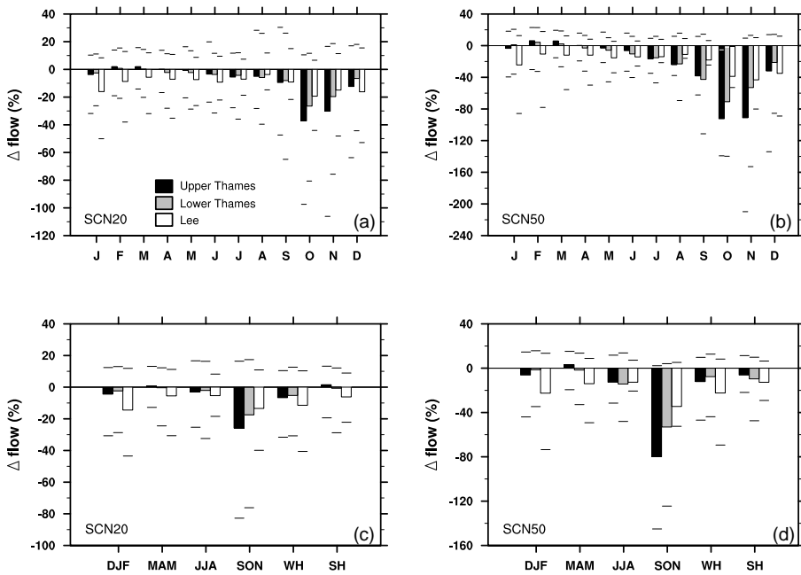
Figure 7. Percentage change in Upper Thames, Lower Thames, Lee catchments for monthly river flows for (a) SCN20, monthly flows, (b) SCN50, monthly flows, (c) SCN20, seasonal flows, (d) SCN50, seasonal flows (standard seasons plus winter half year (WH) and summer half year (SH)). The bars denote the median change from the 100-member ensemble, the upper and lower horizontal lines indicate the ensemble 90th and 10th percentiles, respectively.
