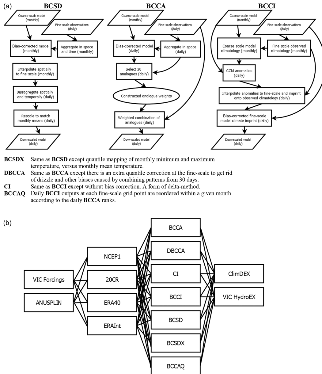
Figure 3. (a) Diagram of the bias corrected spatial disaggregation (BCSD), bias corrected constructed analogues (BCCA), and bias corrected climate imprint (BCCI) downscaling methods and a summary of adjustments made to these methods to create BCSD with monthly minimum and maximum temperature (BCSDX), double BCCA (DBCCA), climate imprint (CI), and BCCA corrected to BCCI (BCCAQ). (b) Workflow diagram for assessment of downscaling techniques in replicating ClimDEX and hydrologic extremes.
