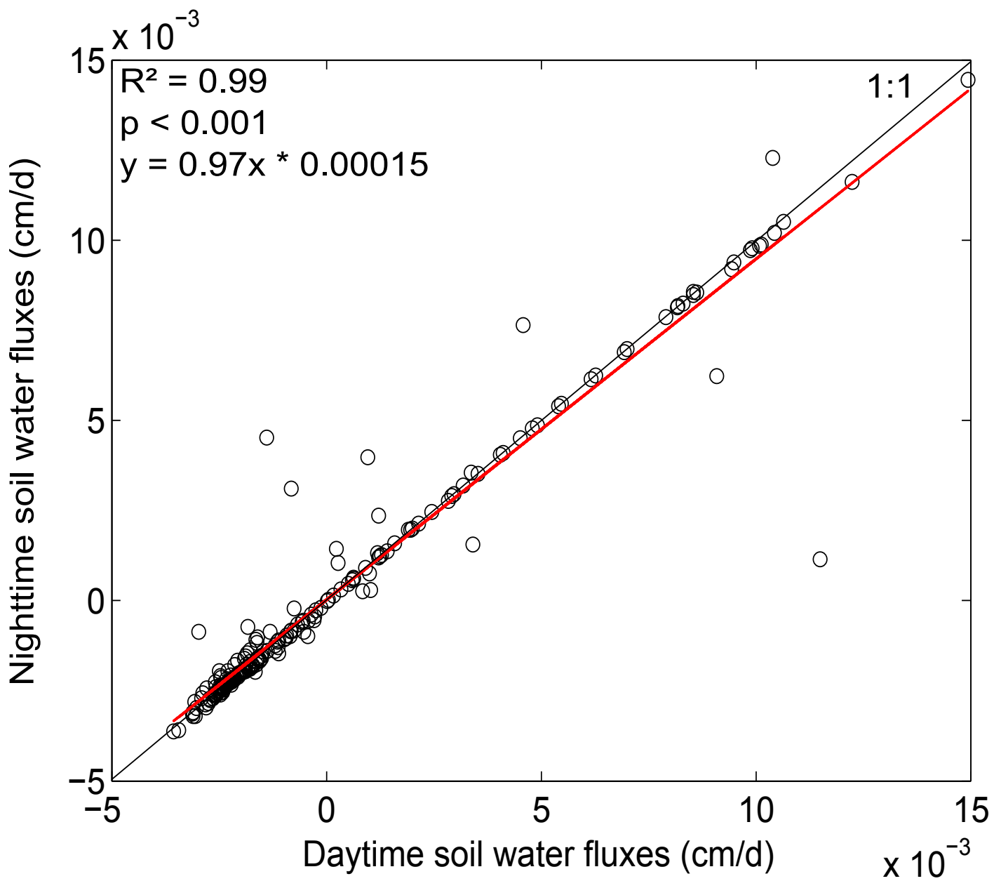
Figure S1: Correlation between simulated mean fluxes of the respective day and the mean fluxes in the nights before and after one particular day. The analysis was conducted with the LinearModel.fit function of the Statistics toolbox in Matlab R2012.b.
