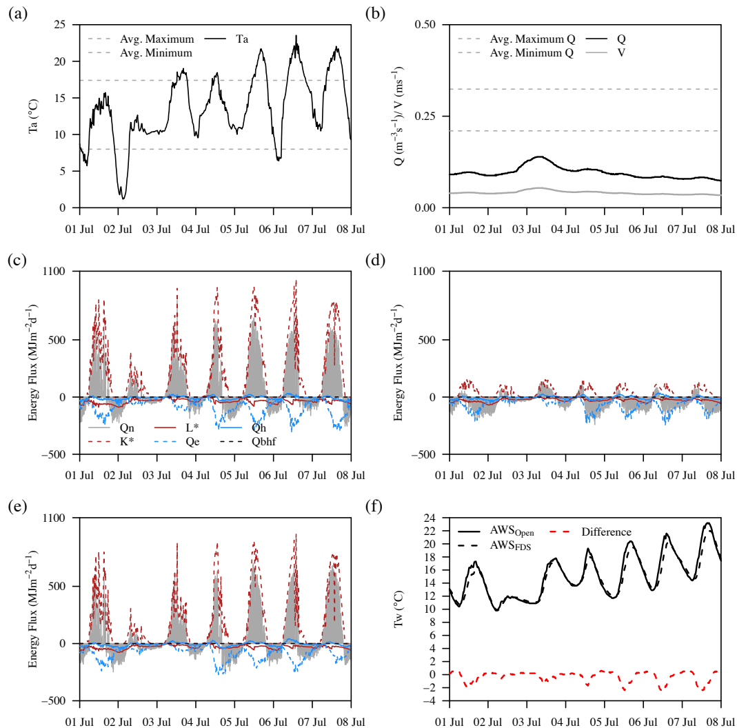
Figure 2. Study period (a) air temperature, (b) discharge and energy fluxes at (c) \text{AWS}_{\text{Open}} , (d) \text{AWS}_{\text{FUS}} , (e) \text{AWS}_{\text{FDS}} and (f) water temperature at \text{AWS}_{\text{Open}} , \text{AWS}_{\text{FDS}} and \text{AWS}_{\text{Open}} minus \text{AWS}_{\text{FDS}} (positive values indicate that temperature \text{AWS}_{\text{Open}} was greater than temperature at \text{AWS}_{\text{FDS}} ). Averages represent values for DOYs (days of the year) 183 to 289 in the 10 years preceding 2013.
