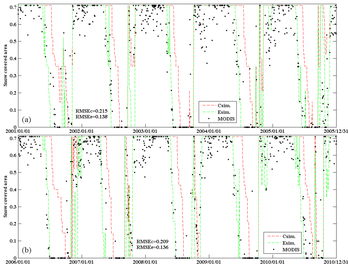
Figure 10. Same as Fig. 9 but for the Innerschloess basin ( 39 \text{ km}^2 ).
