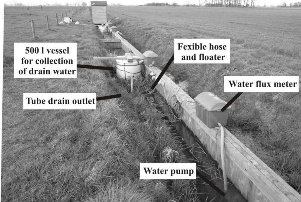
3 Figure S1. Measurement setup with collector vessels for drain discharge, pumps, and water flux 4 meters. The shed in the back houses the data acquisition and control equipment (from Van der 5 Velde et al., 2010).
