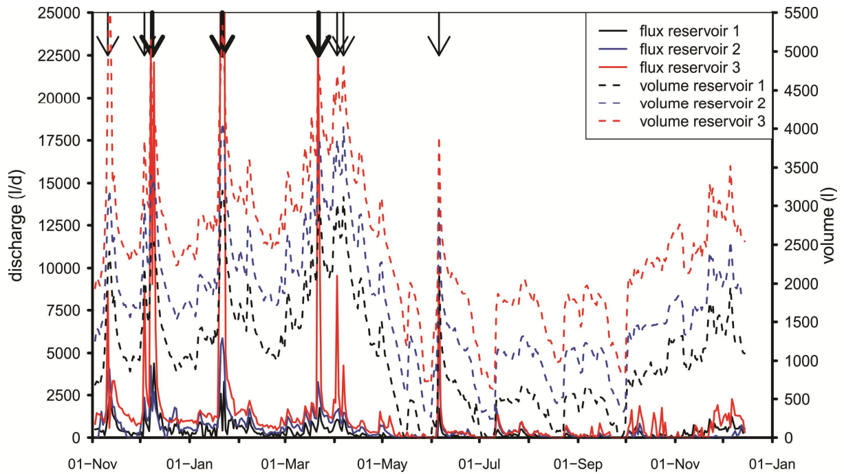
3 Figure S2. Daily average value of hourly measured in-stream reservoir discharge and reservoir 4 volume. Arrows indicate discharge events on which overland flow and interflow towards the 5 reservoirs occurred (bold arrows multiple day events, thin arrows one day events).
