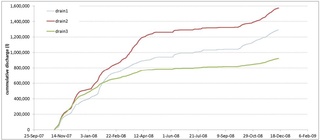
1 2 Figure S4. Measured cumulative discharge of three tube drains, until early Dec. 2007 the 3 discharge of tube drain 3 equals the discharge of tube drain 1. Afterwards, the discharge of tube 4 drain 3 decreases. The increase in Fe concentration of tube drain 3 ends early Dec.
