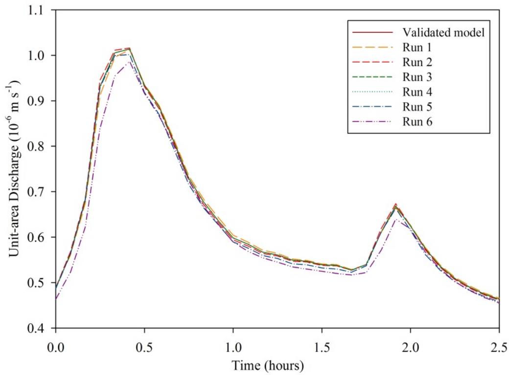
Figure 6. Hydrographs for uncertainty analyses based on variations in sub-catchment width and Manning's n (impervious surface and natural channels) for WS4.
