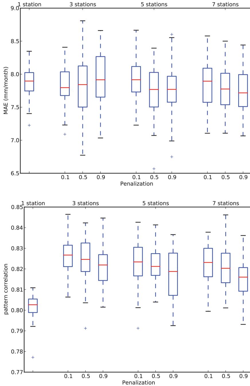
Figure 2: Top: Seasonal Mean Absolute Error between corrected WRF outputs and GHCN. The boxplot encompass 50 perturbed realisations removing a random 10% of the stations each time for various bias correction parameter values. Bottom: as top but for pattern correlation and using AWAP as reference
