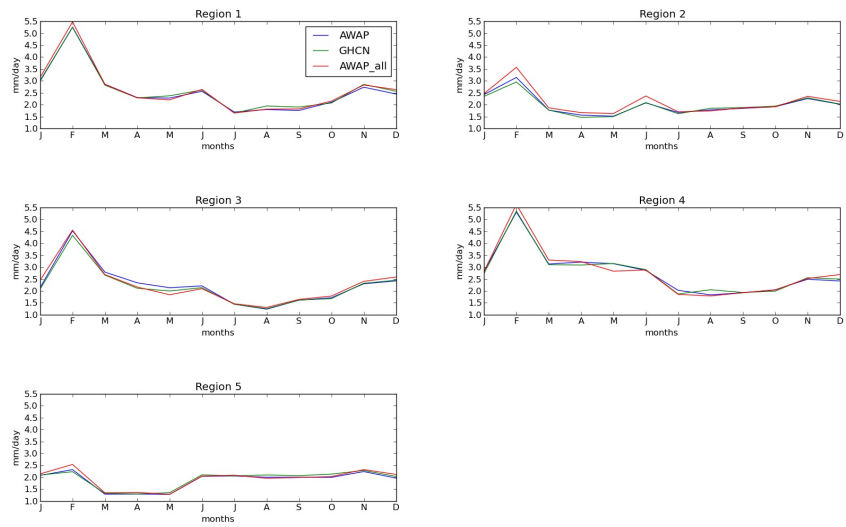
Figure 1: Monthly climatologies using all AWAP grid points within each region (red), all GHCN stations within each region (green), and the nearest AWAP grid point to each station within each region (blue)
