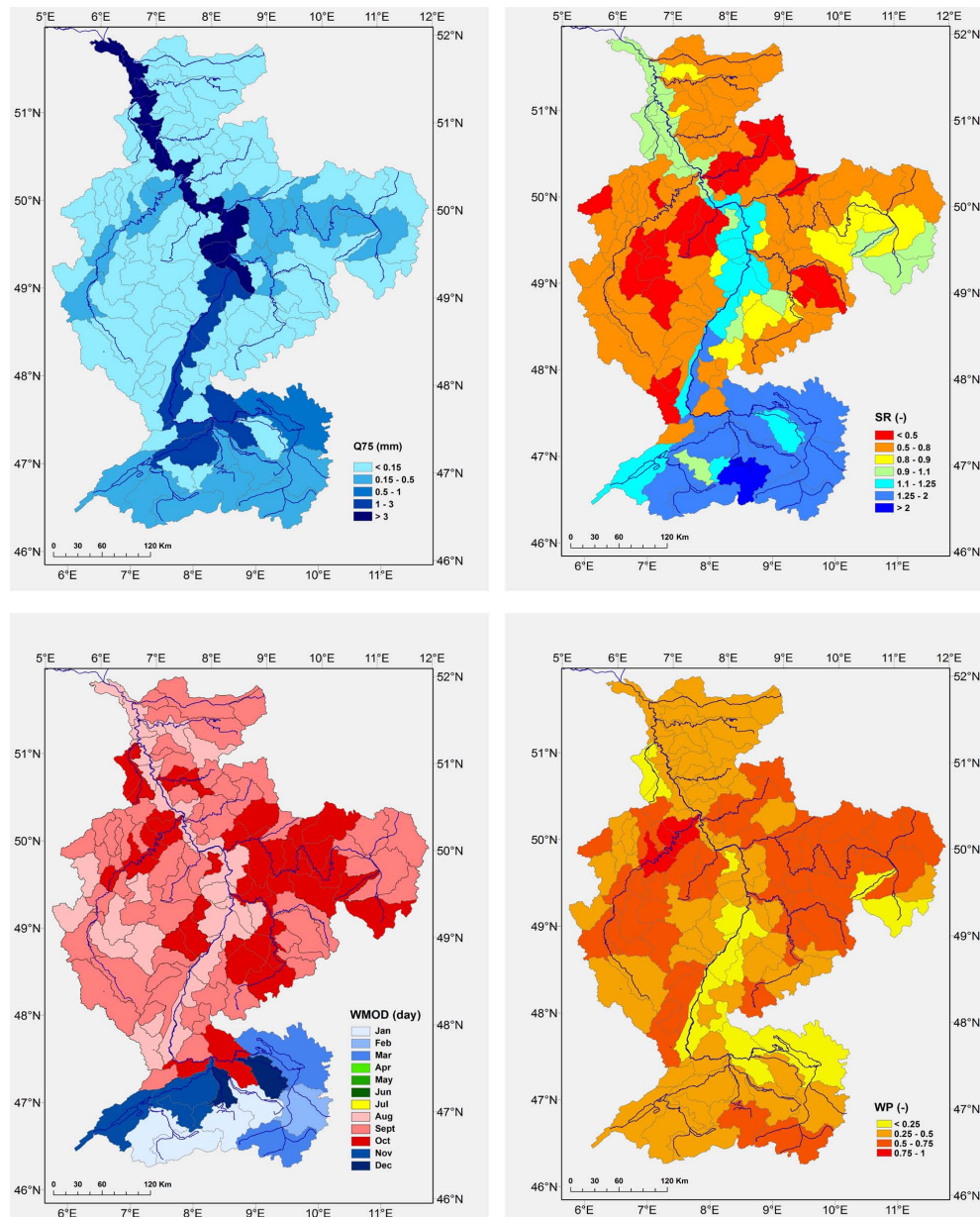
Fig. 3. Low flow threshold ( Q_{75} in \text{mm day}^{-1} and three seasonality indices (SR, WMOD and WP) estimated from simulated low flows using observed climate as model input in 134 sub-catchments for the period 1964–2007 (case 2).
