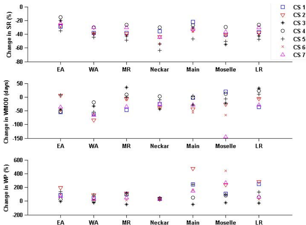
Fig. 6. The relative changes (*) in SR and WP and the changes in WMOD (**) at the outlet of the seven sub-basins estimated from simulated low flows using simulated inputs for the future period 2063–2098 (case 4) compared to simulated low flows using simulated inputs for the reference period 1964–2007 (case 3) from seven climate scenarios (CSs). * (Based on simulated input for future climate – Based on simulated input for current climate)/Based on simulated input for current climate ** Based on simulated input for future climate – Based on simulated input for current climate.
