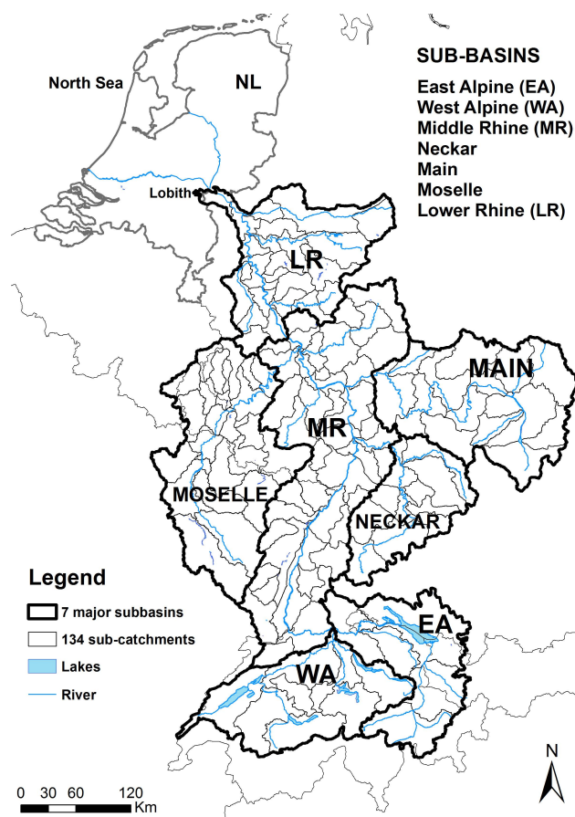
Fig. 1. Schematisation of the 134 sub-catchments (spatial scale of HBV model) and seven major sub-basins of the River Rhine upstream of Lobith.
