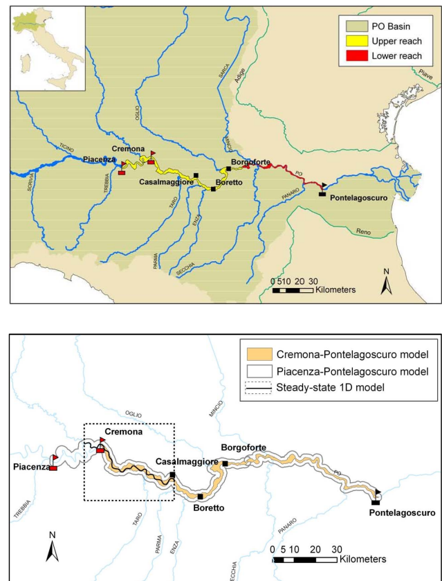
Fig. 1. Po River: upper and lower portions of the study reach; Piacenza, Cremona and Pontelagosuro gauging stations (flags).
