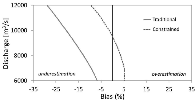
Fig. 7. Bias of Traditional (grey line) and Constrained (dashed line) median rating-curve relative to the normal rating-curve (see Fig. 5).
