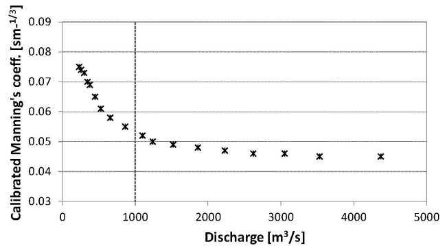
Fig. 3. Variation of calibrated Manning's roughness coefficients ( n ) at the Cremona cross-section in relation to different hydraulic condition (river water discharge).
