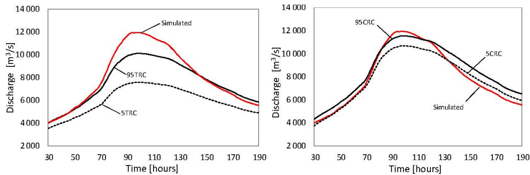
Fig. 9. Cremona cross-section and October 2000 flood: flow hydrograph simulated through the Piacenza-Pontelagoscuoro model (red line); flow hydrographs retrieved from Traditional (left panel) and Constrained (right panel) percentile rating-curves.
