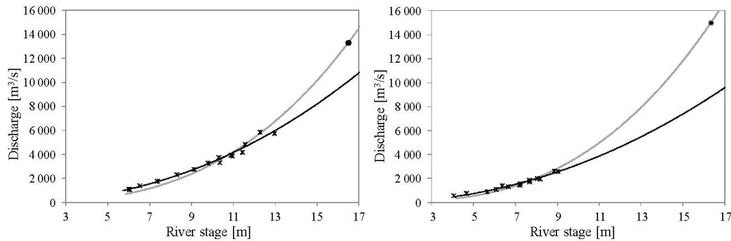
Fig. 4. Cremona cross-section: examples of synthetic measurement campaigns (stars); estimated maximum discharge capacity at Cremona cross-section ( h_{\max} - Q_{\max} , black point); Traditional (black line) and Constrained (grey line) rating-curves.
