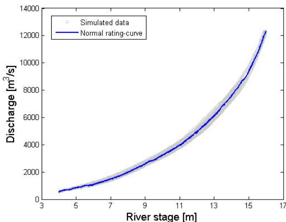
Fig. 5. Cremona cross-section: simulated h(t) - Q(t) pairs for 10 historical flood events (grey dots) adopting the calibrated Piacenza-Pontelagoscuo quasi-2-D model; normal rating-curve (blue line).
