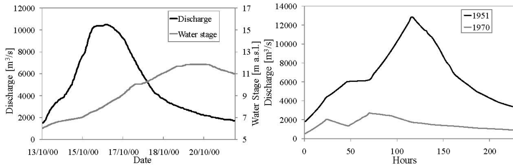
Fig. 2. Boundary conditions for the hydraulic modelling. October 2000 flood event: flow hydrograph and stage hydrograph observed at Piacenza and Pontelagoscuoro, respectively (left panel). Examples of historical flow hydrographs observed at Piacenza and used for generating synthetic measurement campaigns (right panel).
