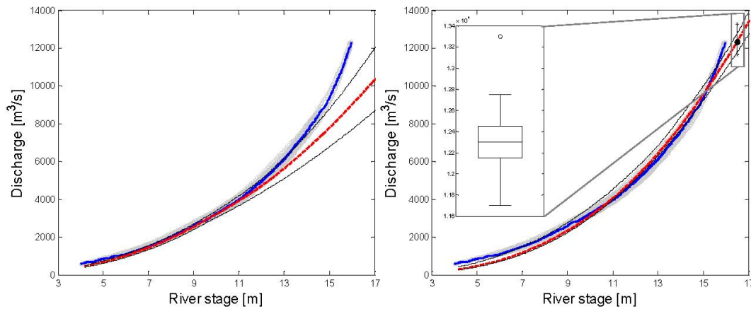
Fig. 6. Cremona cross-section: normal rating-curve (blue line); median rating-curve (red dashed line) for Traditional (left panel) and Constrained (right panel) approaches and corresponding 90 % confidence intervals (black lines); for the Constrained approach the diagram also reports the average h_{\max} - Q_{\max} pair (black point), range of simulated values (bands) and a detailed representation of all h_{\max} - Q_{\max} pairs (box-plot).
