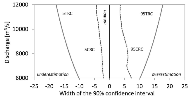
Fig. 8. Width of 90 % confidence intervals for Traditional (5TRC and 95TRC, grey lines) and Constrained (5CRC and 95CRC, dashed lines) rating-curves.
