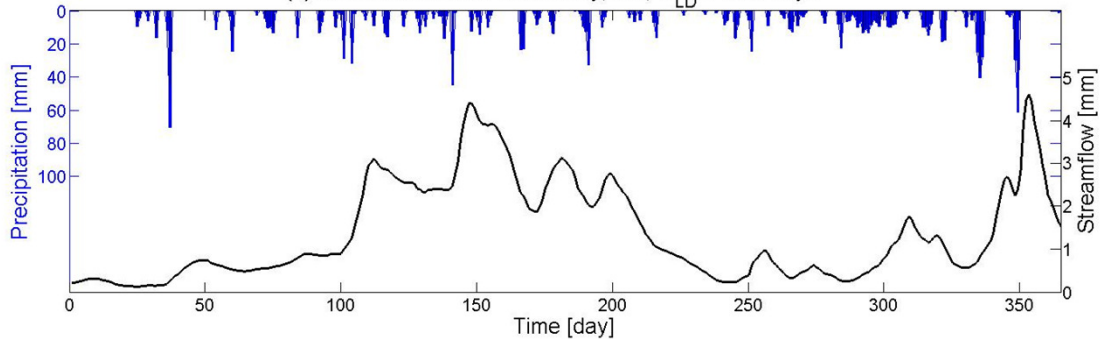
(b) Indian Creek near Laboratory, NC, R_{LD} = 0.15 \text{ days}^{-1}
