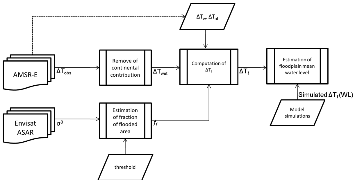
Fig. 5. Flow diagram of the methodology.
