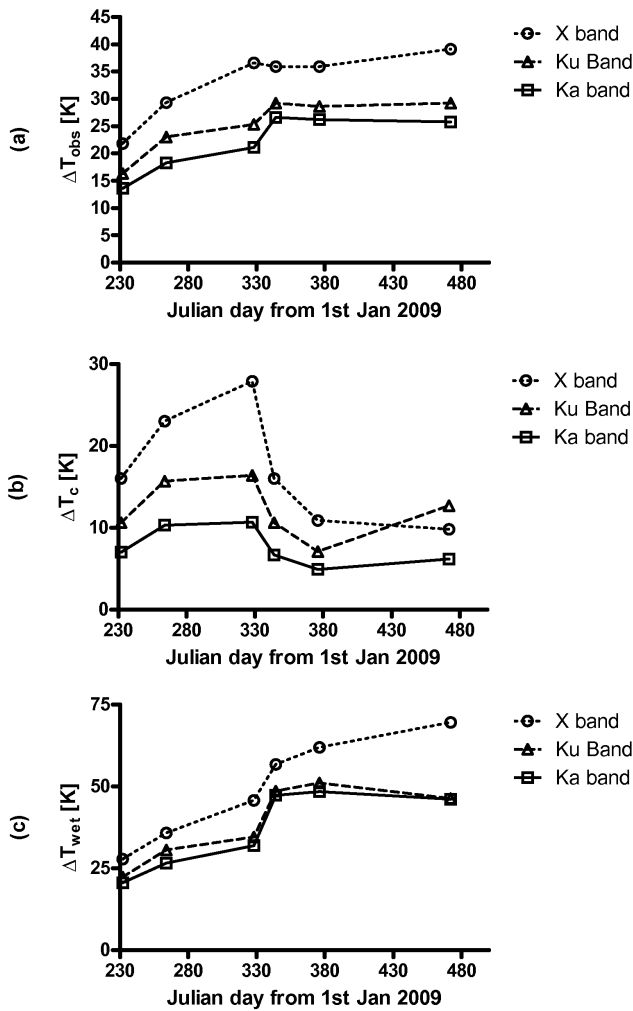
Fig. 9. Polarization differences as a function of time for the three AMSR-E considered bands. (a): overall measured \Delta T_{obs} (b): continent \Delta T_c . (c): wetland \Delta T_{wet} .
