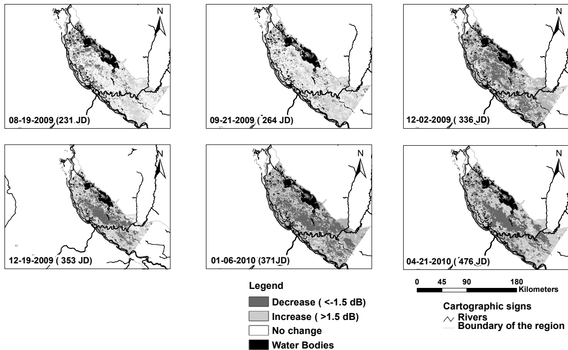
Fig. 7. Maps of \sigma^0 change derived from ASAR images for six dates. Julian dates starting from 1 January 2009: 231, 264, 336 (top figures), 353, 371, 476 (bottom figures).
