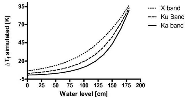
Fig. 6. Polarization difference in flooded marsh ( \Delta T_f ) simulated as a function of water level at X, Ku and Ka band.
