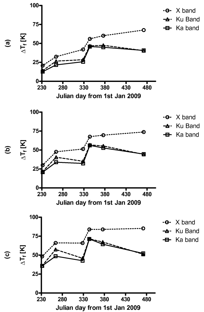
Fig. 10. \Delta T_f as a function of time for the three frequencies and for three different thresholds. (a) 1 dB, (b) 1.5 dB and (c) 2 dB
