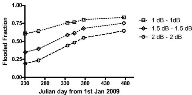
Fig. 8. Fraction of flooded area estimated from ASAR images for six dates and three different thresholds
