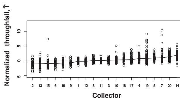
Fig. 2. Plot of normalized throughfall, \tilde{T} , for the whole period. Each circle represents the event throughfall volume at a single collector, normalized to zero median and unit variance for that event. The collectors are plotted on the horizontal axis and ranked by their means, \tilde{T} , which are connected by the black curve.
