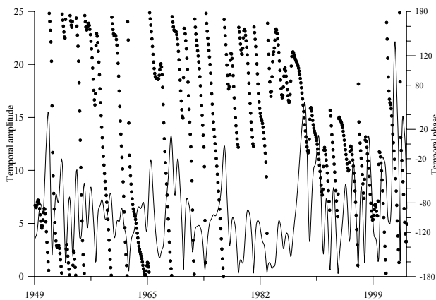
Fig. 5a. The normalized temporal coefficient (amplitude in solid line and phase in solid circles) of the CEOF pattern of the Mean Monthly Temperature anomalies.
