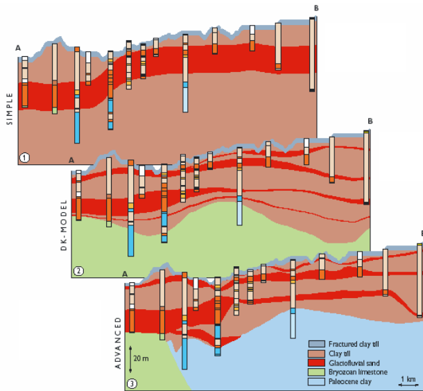
Fig. 1. Geological complexity and simulated age distribution. In a simple (upper), in an intermediary (middle), and in a complex hydrogeological conceptual model (lower). From Troldborg (2000).
