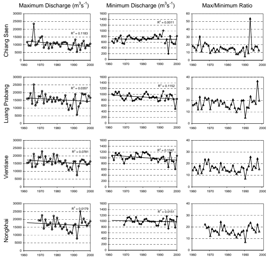
Fig. 4a. Comparisons of maximum, minimum discharge and maximum/minimum ratios at four stations (Chiang Saen, Luang Prabang, Vientiane and Nongkhai) in the upper portion of the study area.
