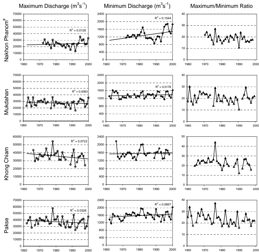
Fig. 4b. Comparisons of maximum, minimum discharge and maximum/minimum ratios at four stations (Nakhon Phanom, Mukdahan, Khong Chiam and Pakse) in the lower portion of the study area.
