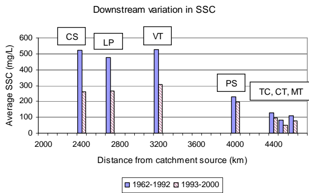
Fig. 8. Sediment concentration variation along the Lower Mekong.
