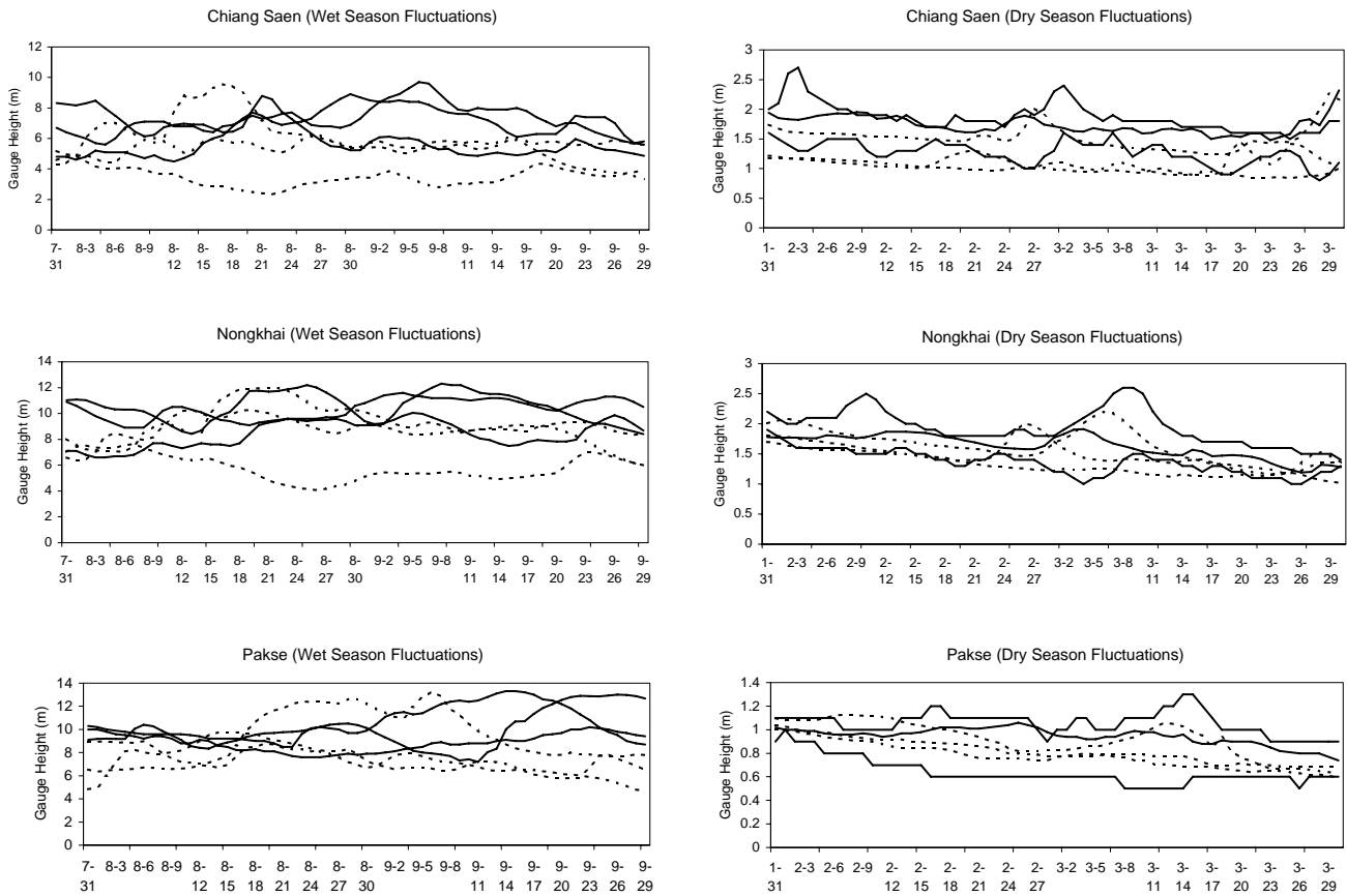
Fig. 5. Comparisons of pre- and post-dam wet season and dry season fluctuations at three stations (Chiang Saen, Nongkhai, and Pakse). Pre-dam years (1988, 1991, 1992) are depicted by dotted lines and post-dam (1996, 1999, 2000) years are depicted by solid lines.
